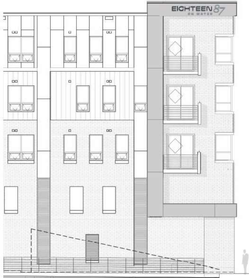
proposed west elevation - day view
