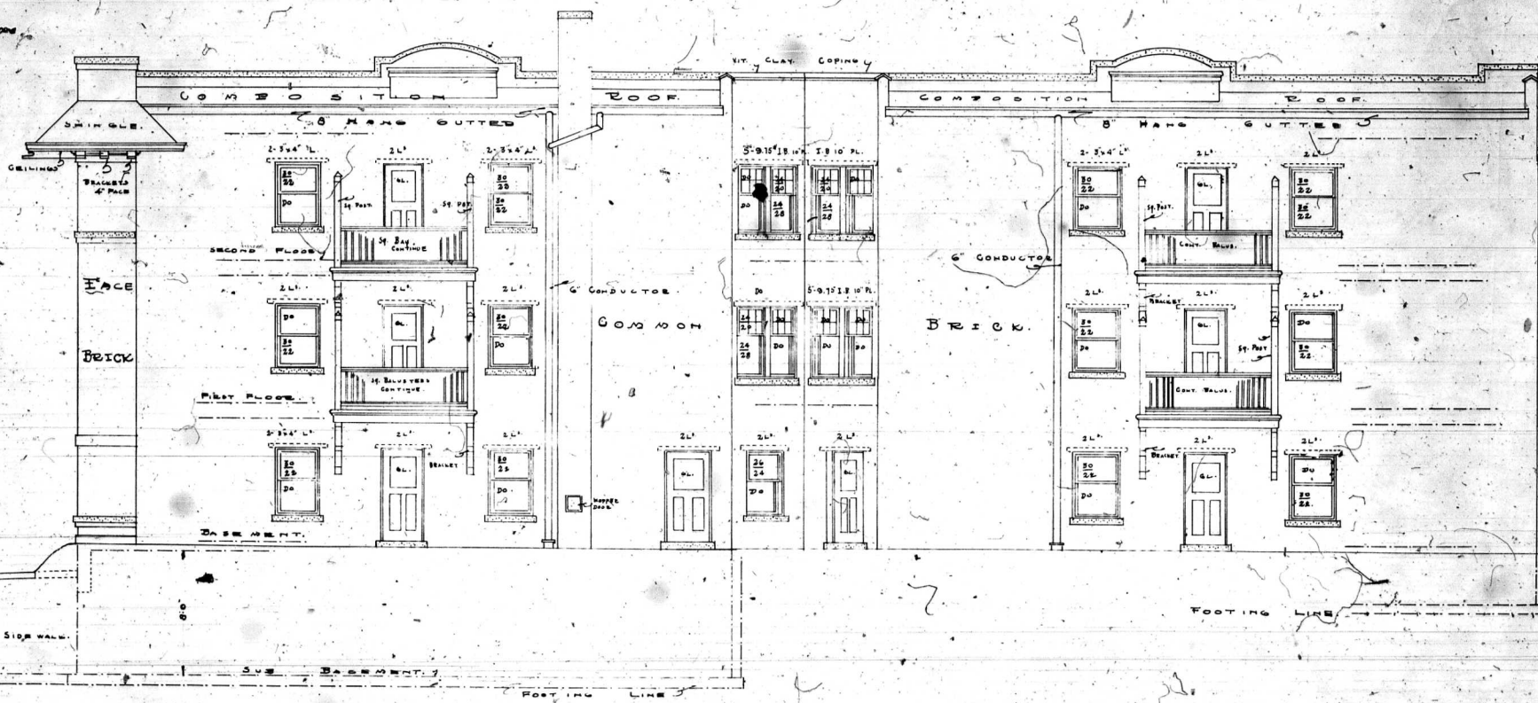
REAR ELEVATION W. HOFFMAN
