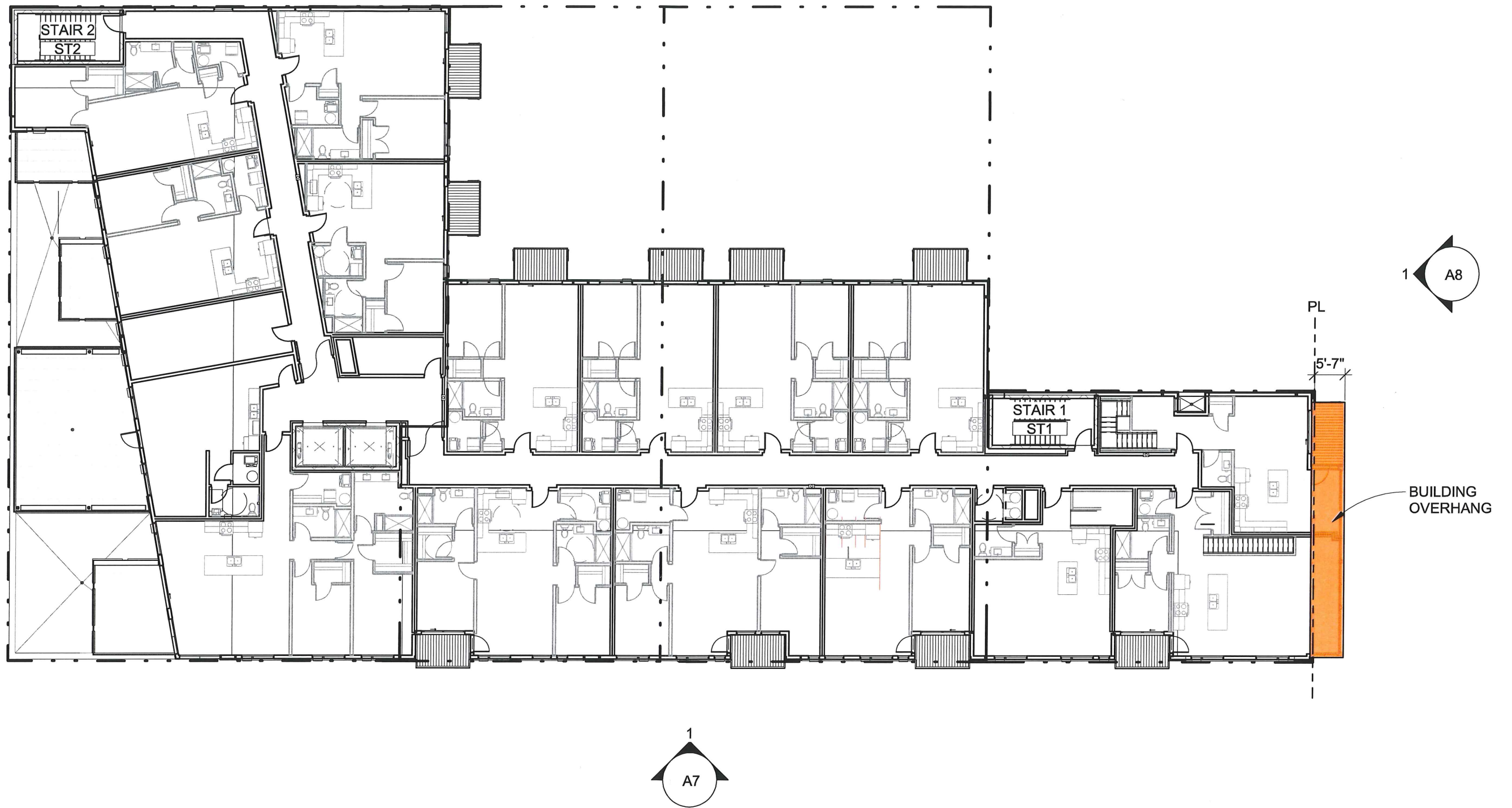
1 LEVEL 4 FLOOR PLAN 1" = 20'-0"
