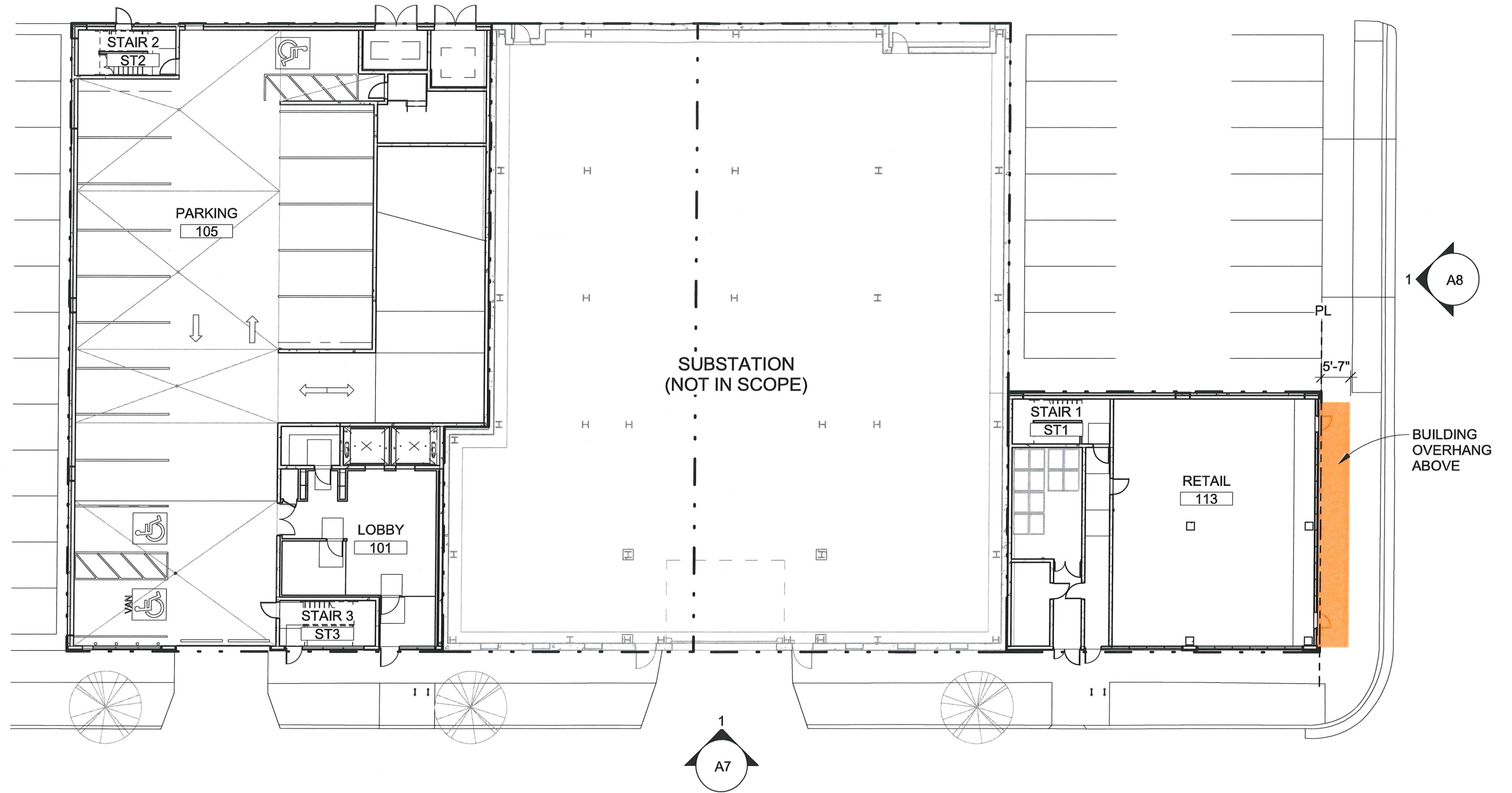
1 LEVEL 1 FLOOR PLAN 1" = 20'-0"
