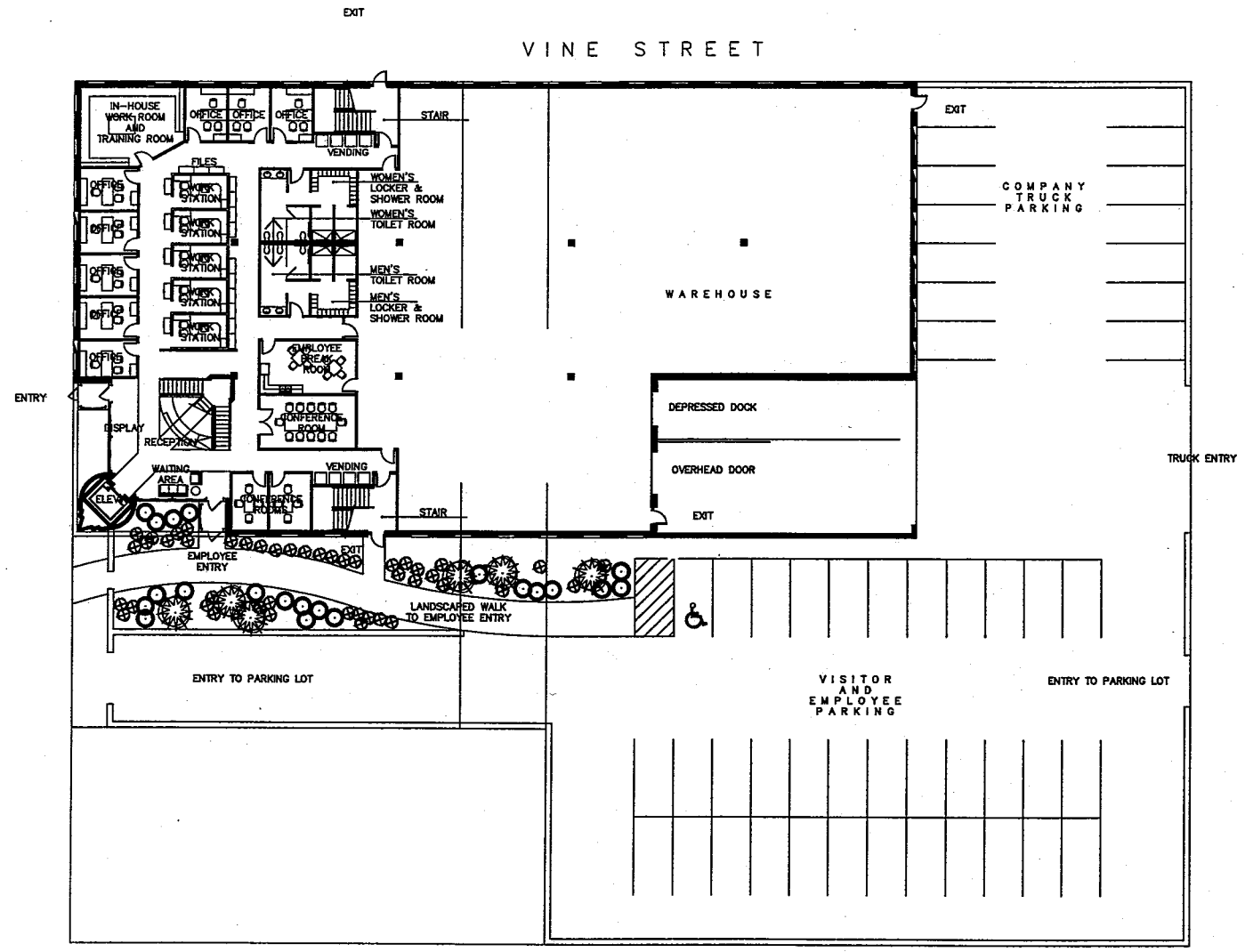
1 PROPOSED FIRST FLOOR / SITE PLAN SCALE: 1/16" = 1'-0"
