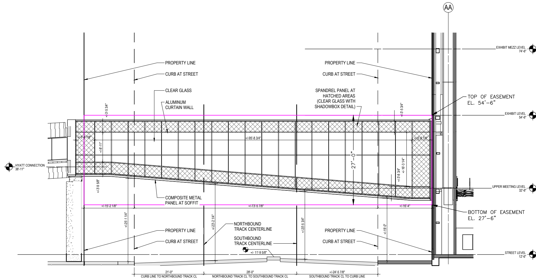
1 VEL R. PHILLIPS AVE SKYBRIDGE AIR RIGHTS EASEMENT SECTION NOT TO SCALE
