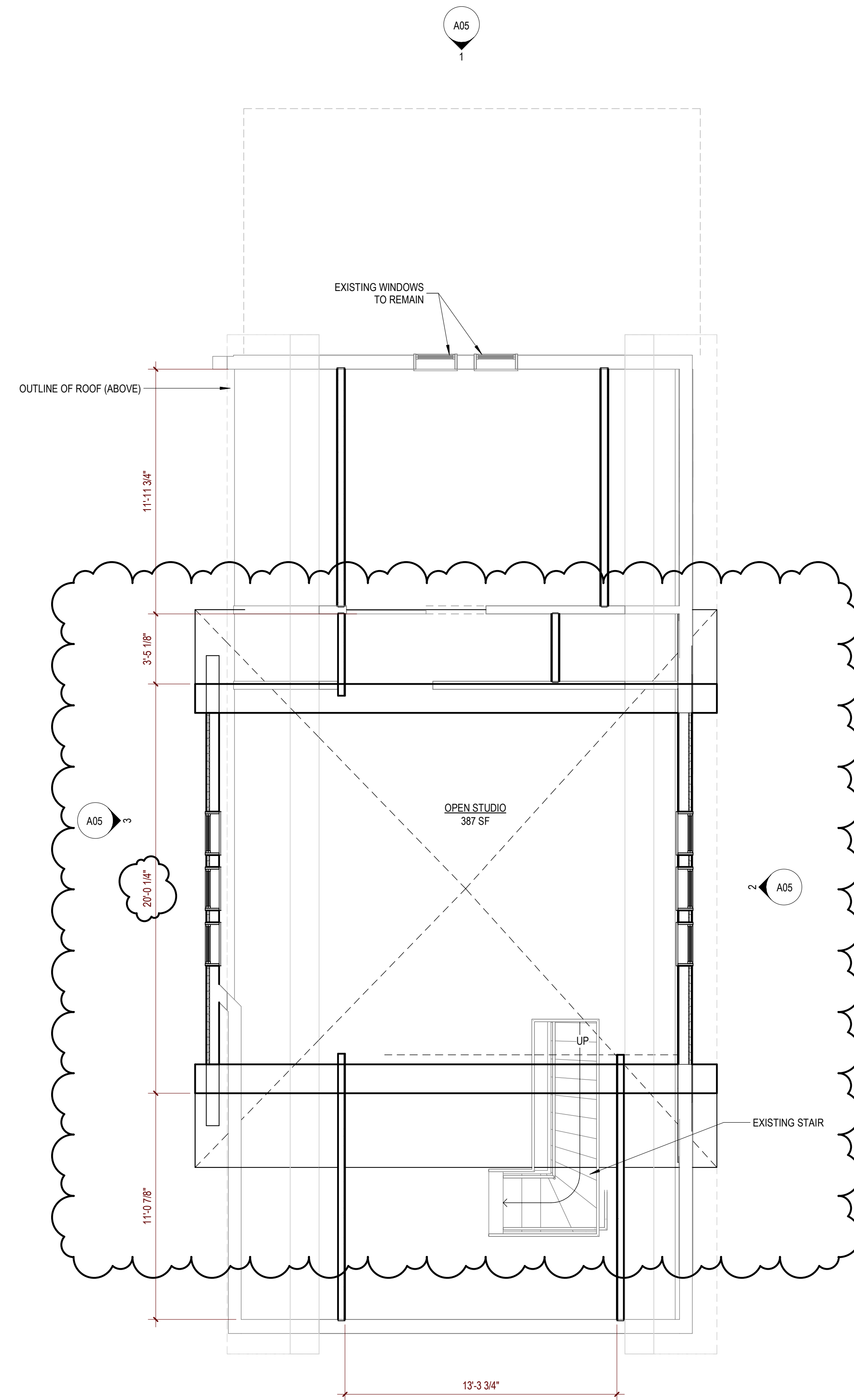
3 THIRD FLOOR RENOVATION 1/4" = 1'-0"
