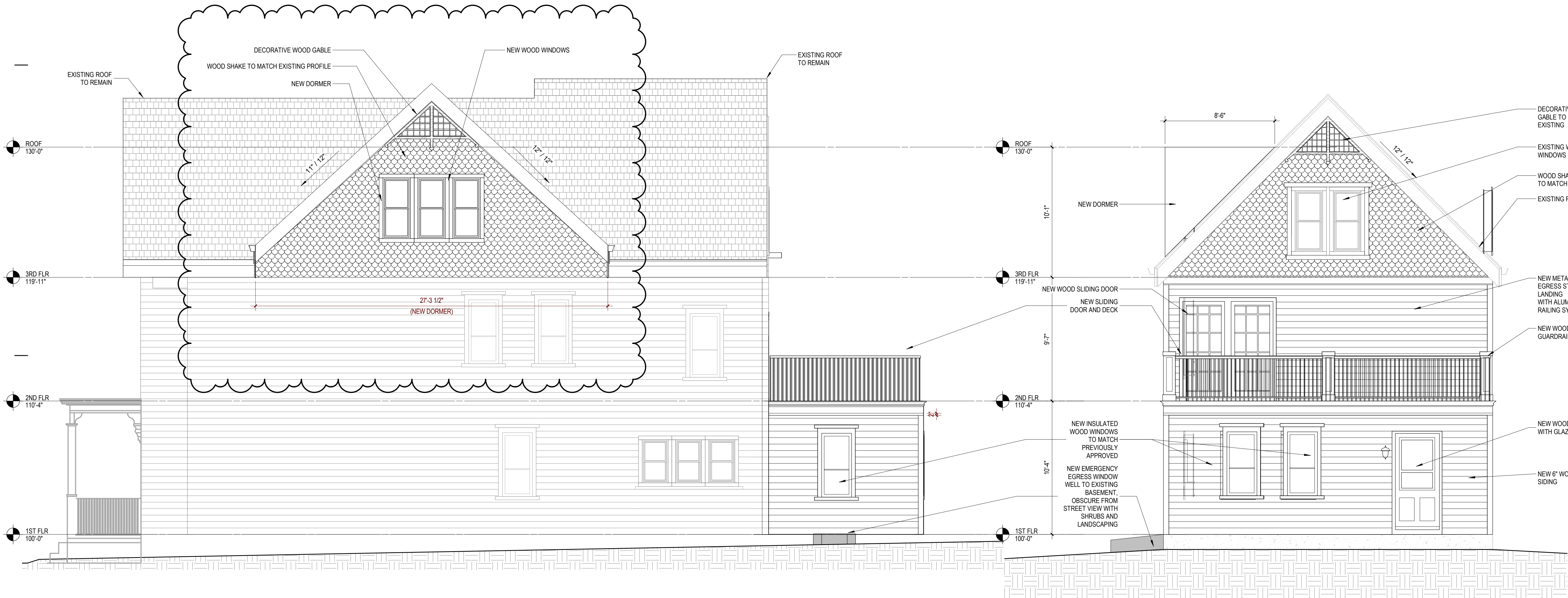
2 EAST ELEVATION 1/4" = 1'-0"
