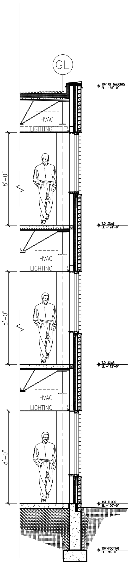
Class C Office Space 1/2" = 1'-0"
