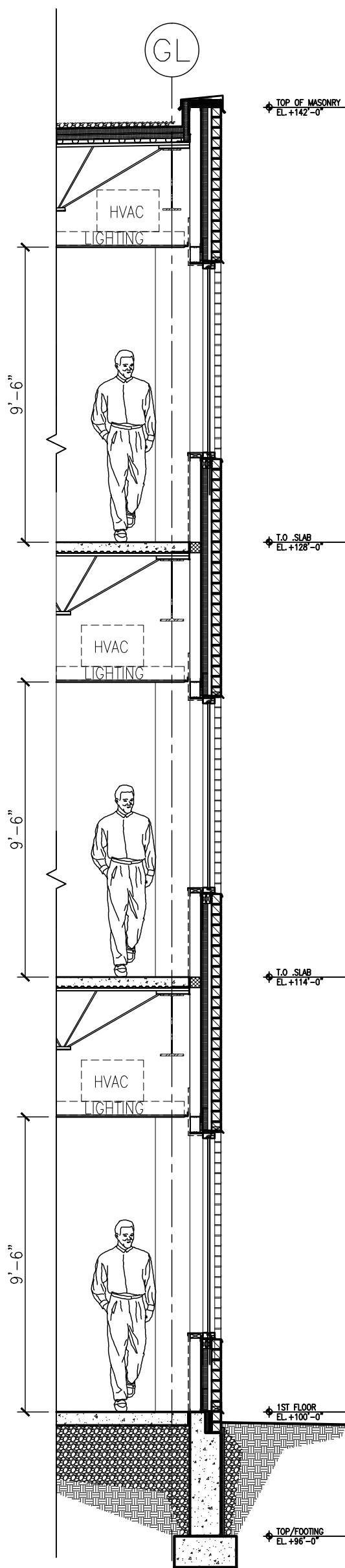
Class A Office Space 1/2" = 1'-0"
