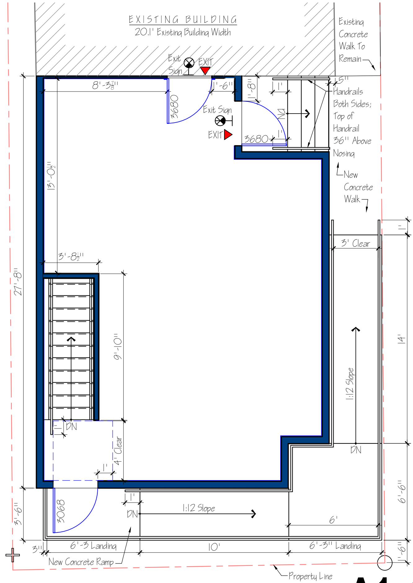
SITE PLAN/FIRST FLOOR PLAN 1/4" = 1'-0"
