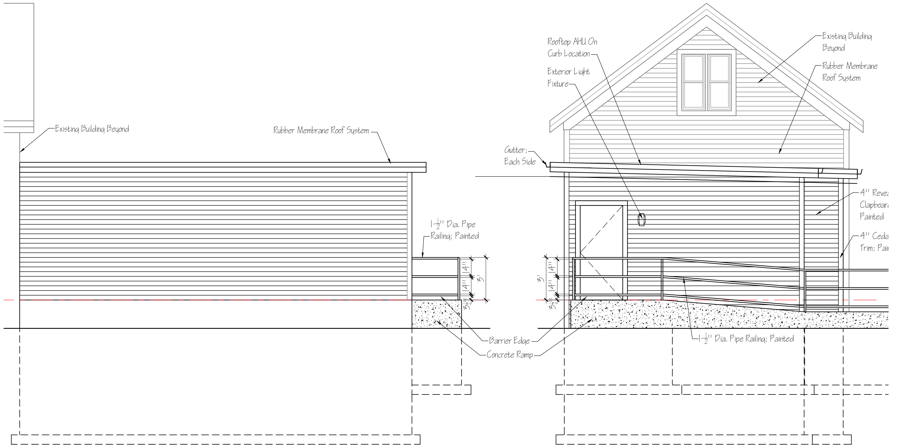
WEST (SIDE) ELEVATION 1/4" = 1'-0"
