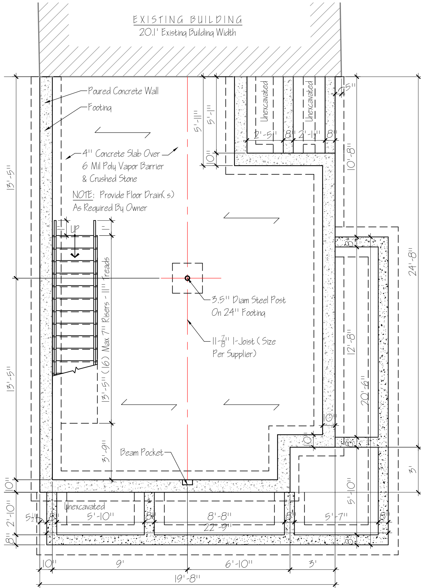
FOUNDATION PLAN 1/4" = 1'-0"
