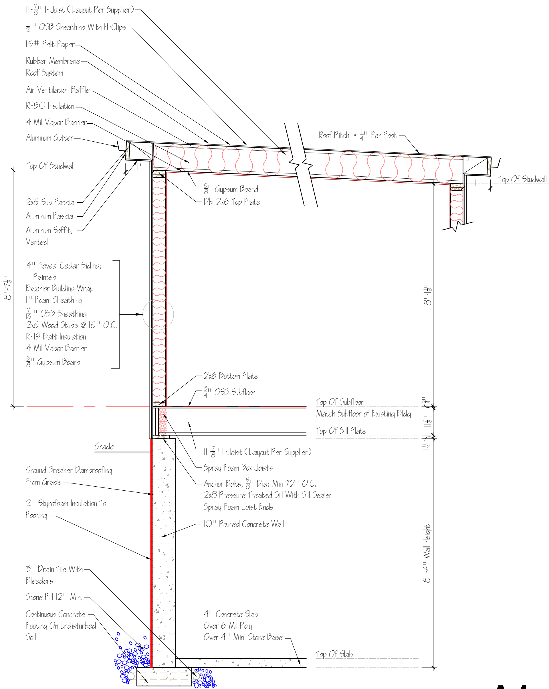
WALL SECTION 1/2" = 1'-0"
