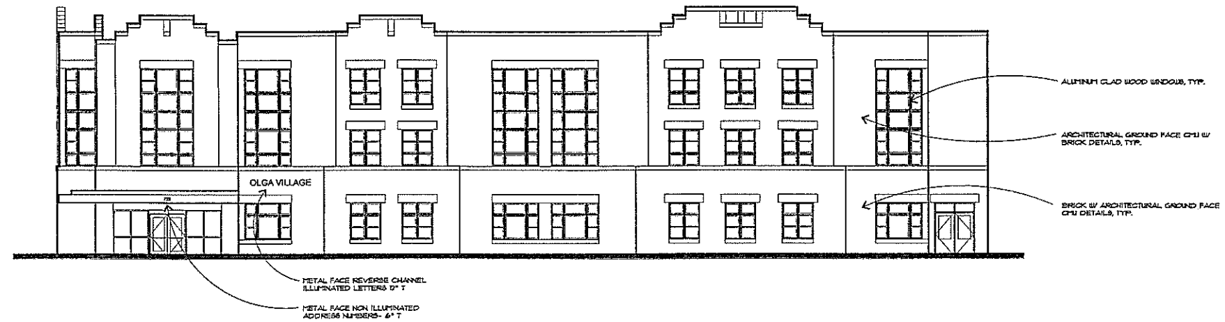
SOUTH ELEVATION 1/8"=1'-0" 3
