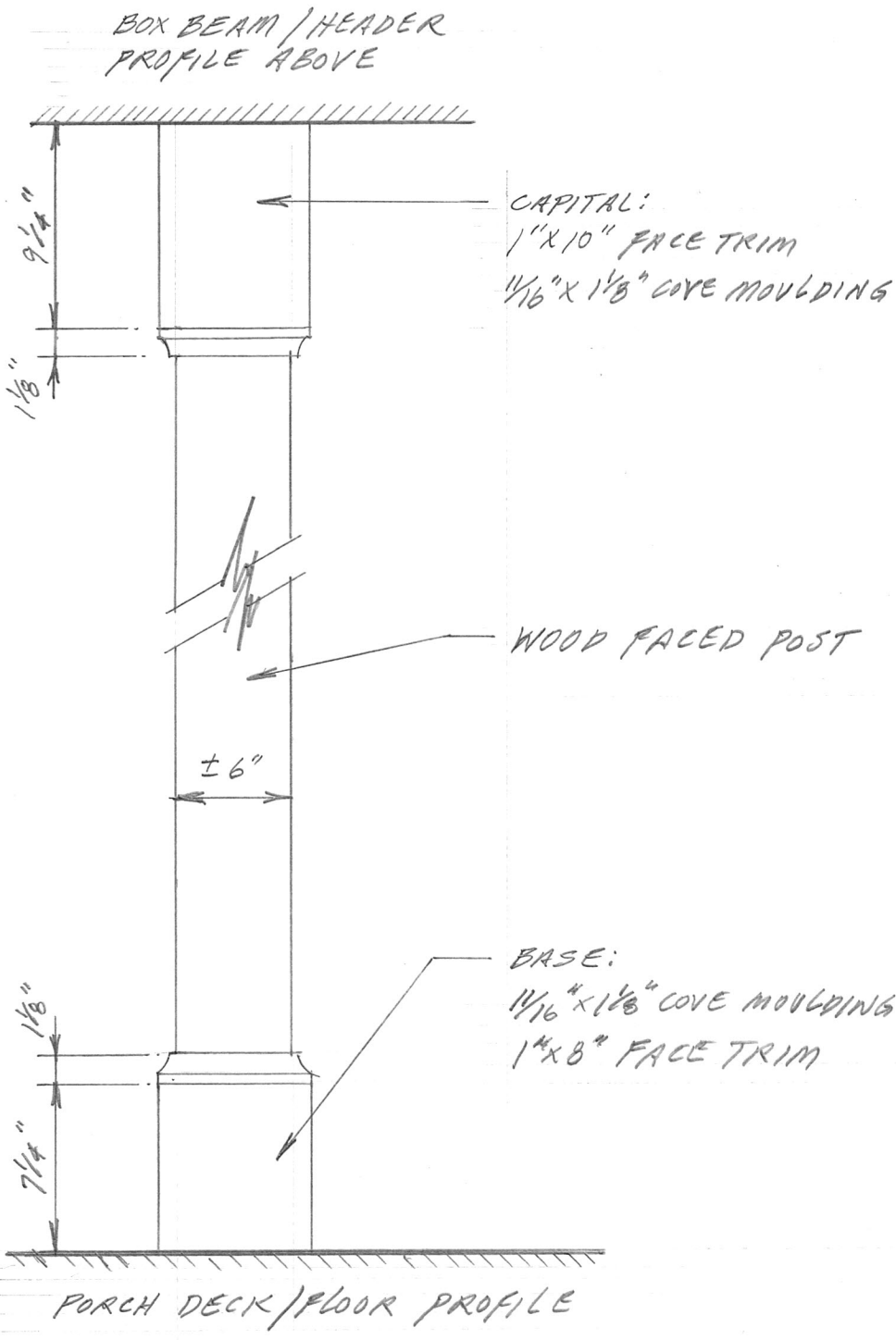
WOOD COLUMN DETAIL PAINTED FINISH
