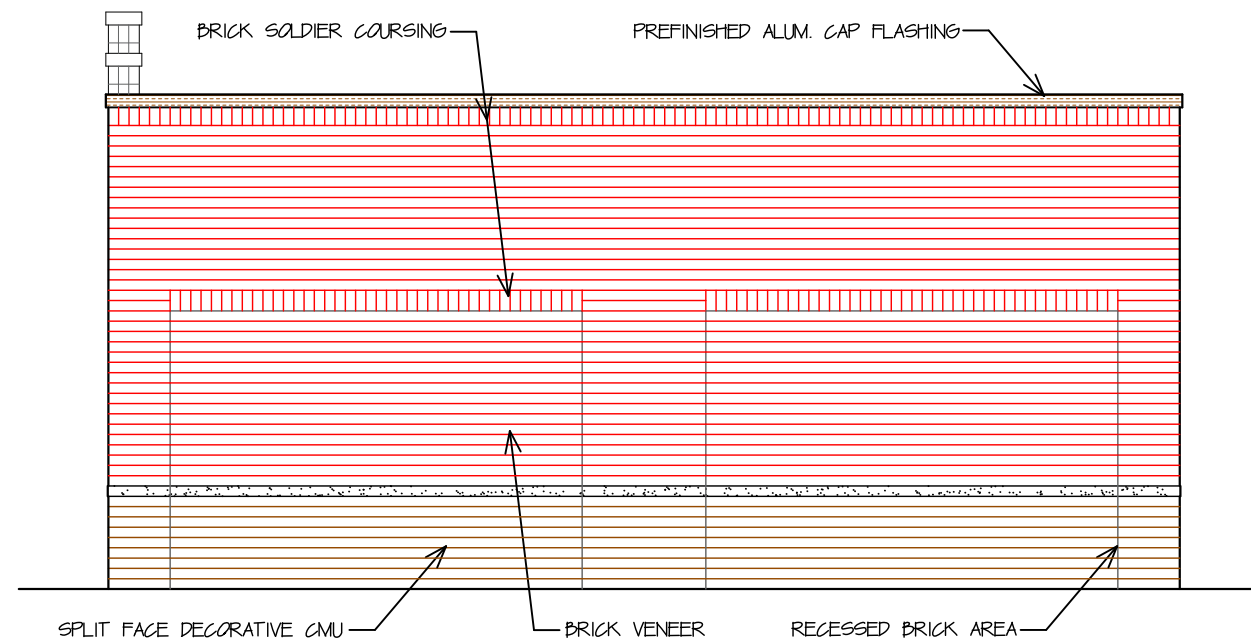
EAST ELEVATION
