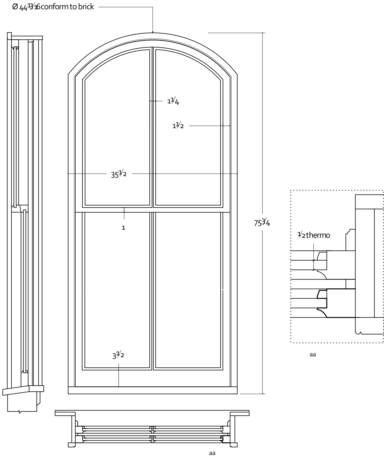
Proposed wood sash replacement for the 2nd floor front facade at 2015 North Palmer Street Milwaukee Wis. Color: Sherwin Williams Hartford Green or equal.
