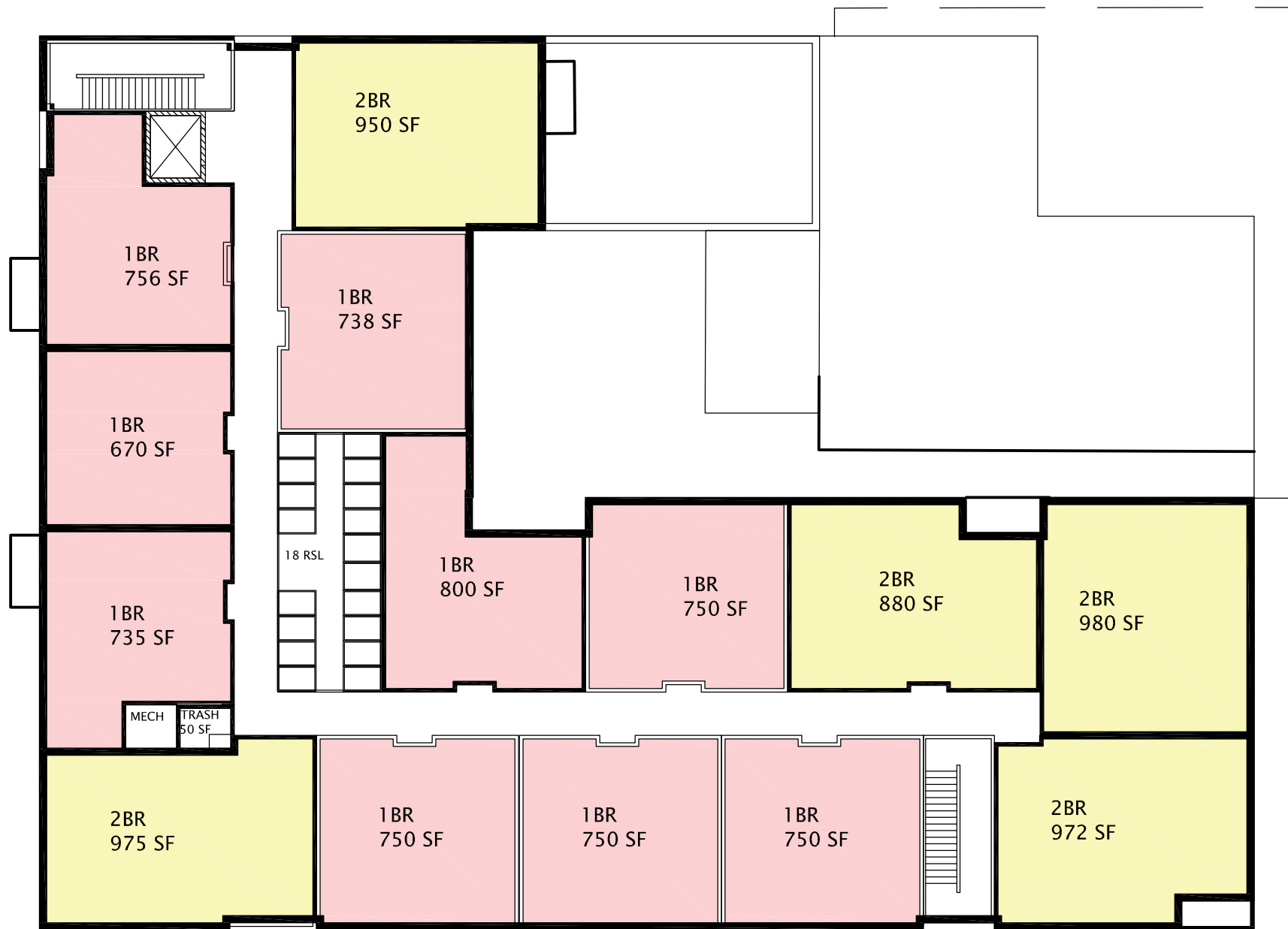
BUILDING A – THIRD AND FOURTH FLOOR PLAN
