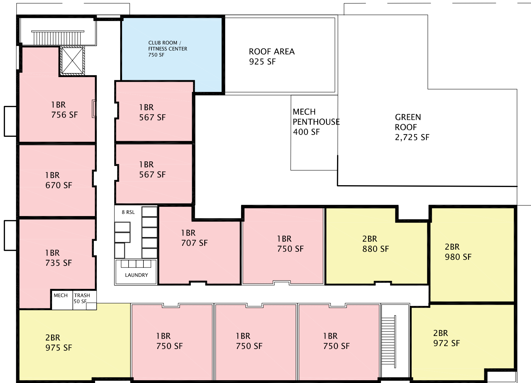
BUILDING A – SECOND FLOOR PLAN
