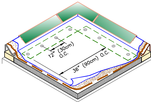
CORNER REINFORCEMENT
