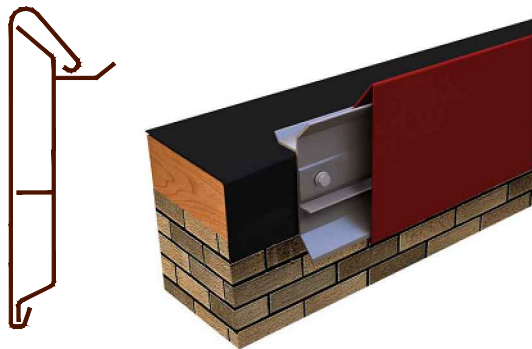
VERSITRIM EX SNAP-ON FASCIA
