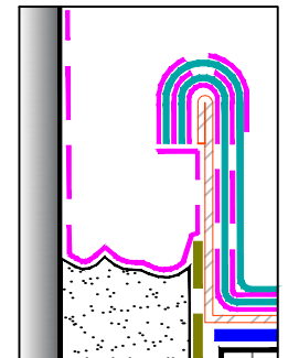
MANDATORY EPDM PRIMER AT ALL INTERFACES OF POURABLE SEALER
