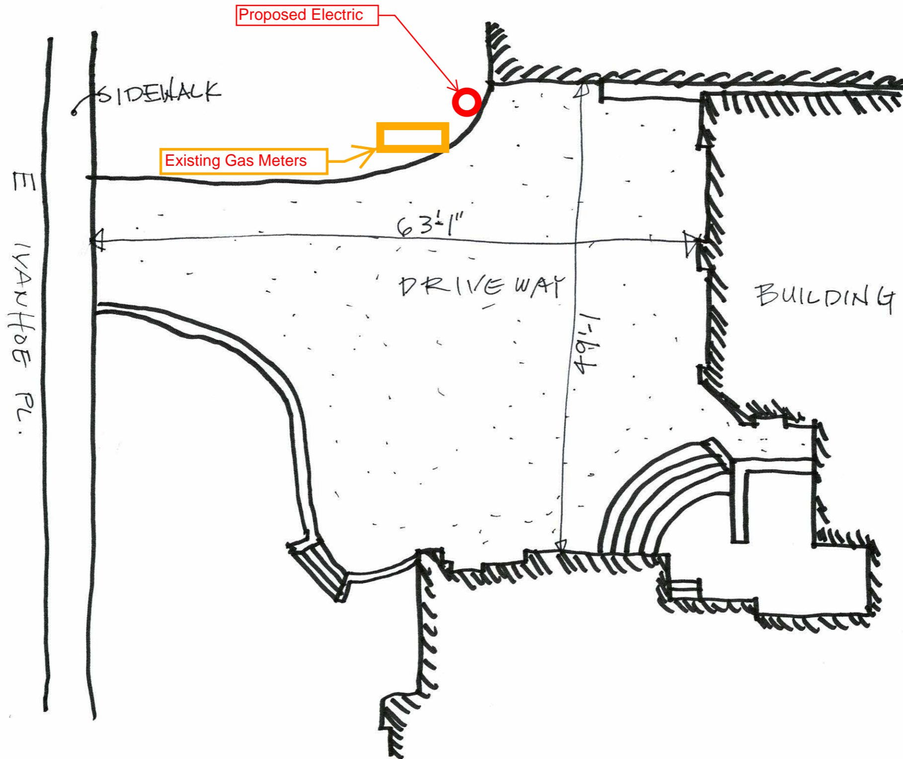
SITE PLAN - AS BUILT
