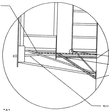
3 DETAIL "A" 1/4" = 1'-0"
