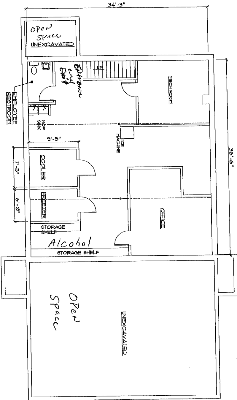
1 Existing Basement Floor Plan A-2 Scale: 3/32" = 1'-0"
