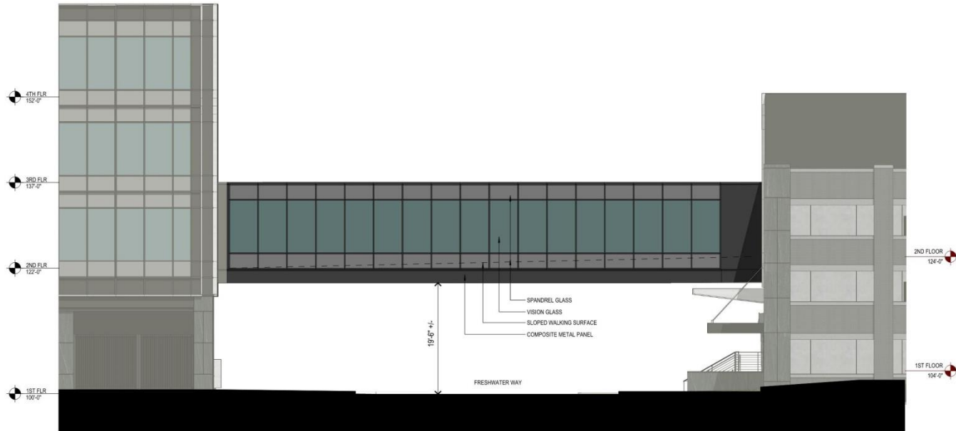
2 WEST ELEVATION 1/8" = 1'-0"
