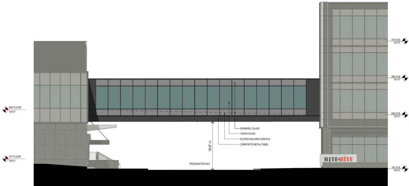
1 EAST ELEVATION 1/8" = 1'-0"
