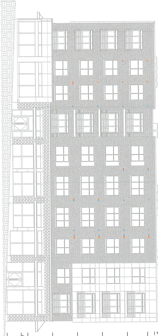
2 SOUTH ELEVATION SCALE: 1/8"=1'-0"
