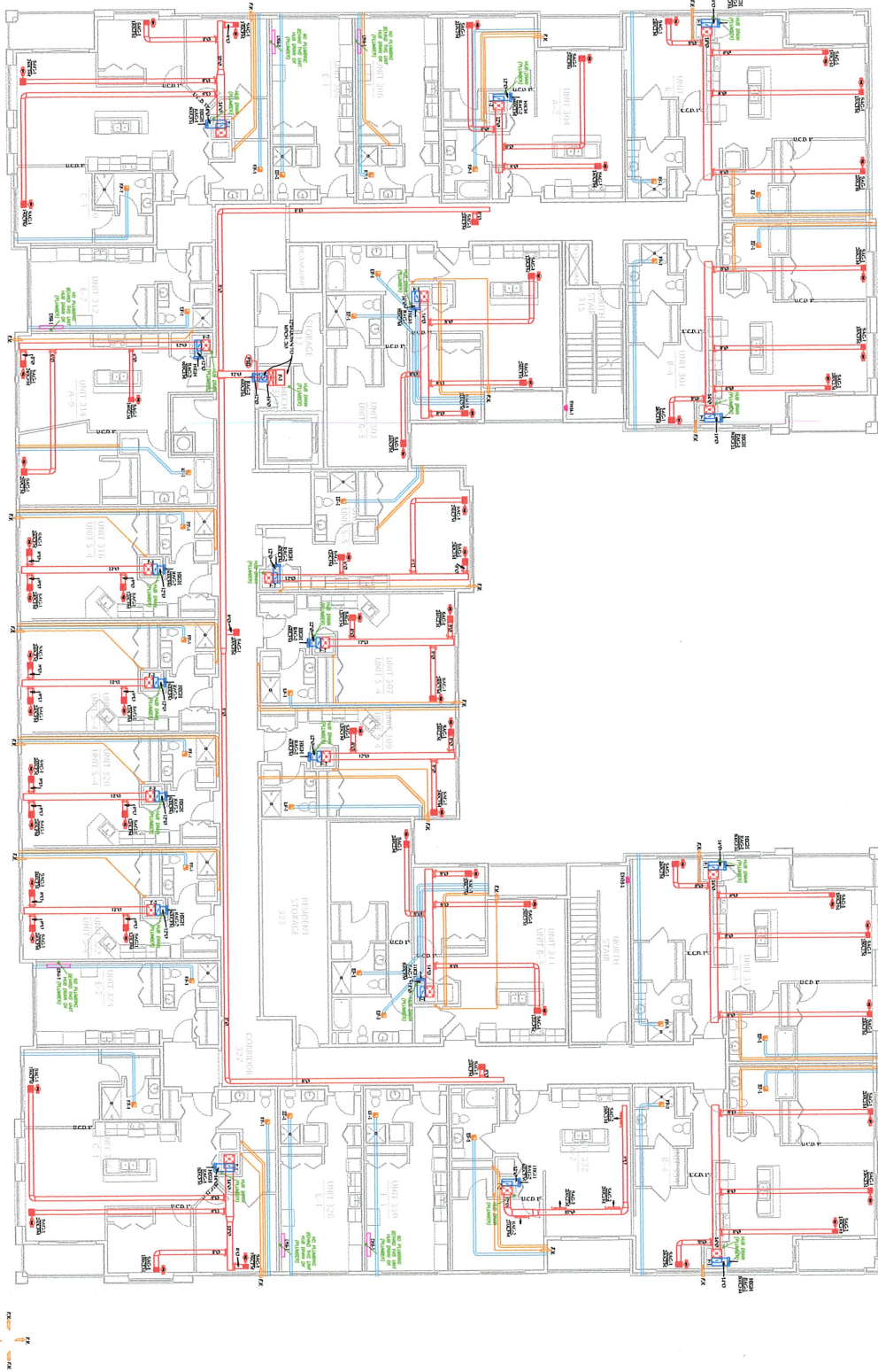
1 THIRD FLOOR HVAC LAYOUT M3 SCALE: 1/8"=1'-0"
