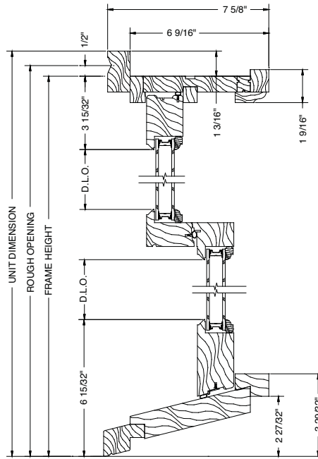
SILL
