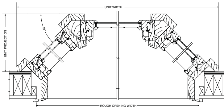
45° Horizontal Section
