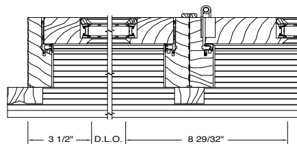
Horizontal Section
