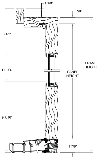
Vertical Section
