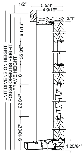
6'-8" EXAMPLE HEIGHT ALUMINUM WEEP SILL Raised panel
