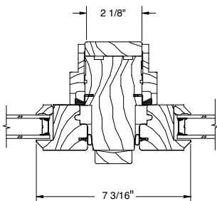
Push-out Awning Standard Mullion
