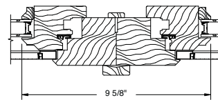
Mullion
