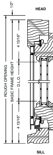
Vertical Section
