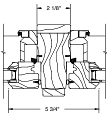
Crank-Out Awning Standard Mullion
