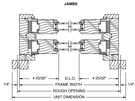
Horizontal Section
