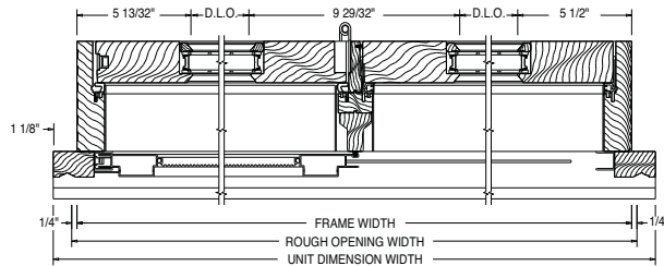
Horizontal Section
