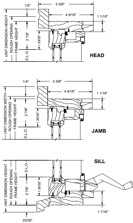
Crank-Out Casement
