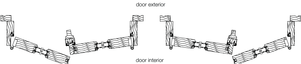
AL (French, Hinged Left, Active)
