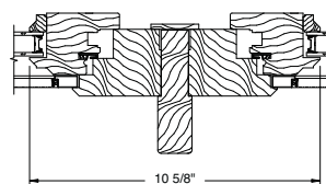
Mullion
