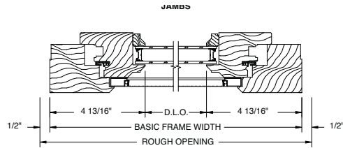
Horizontal Section
