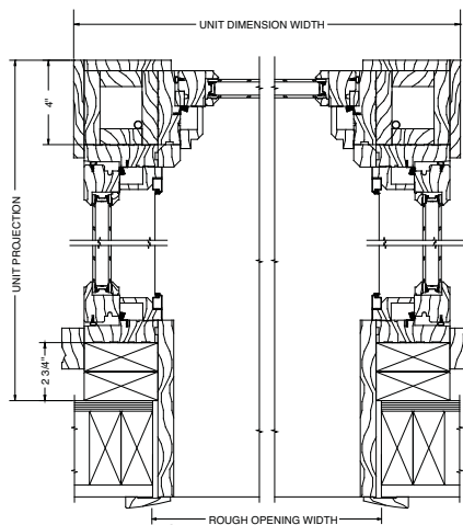
90° Horizontal Section
