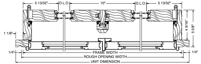
Horizontal Section
