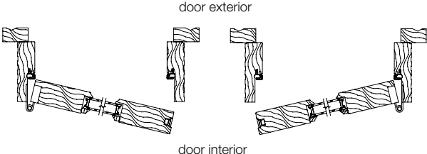
HL (Hinged Left)
