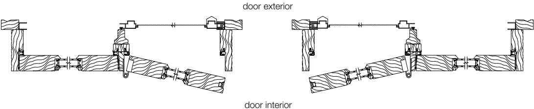
SAL (Stationary, Active Hinged Left)
