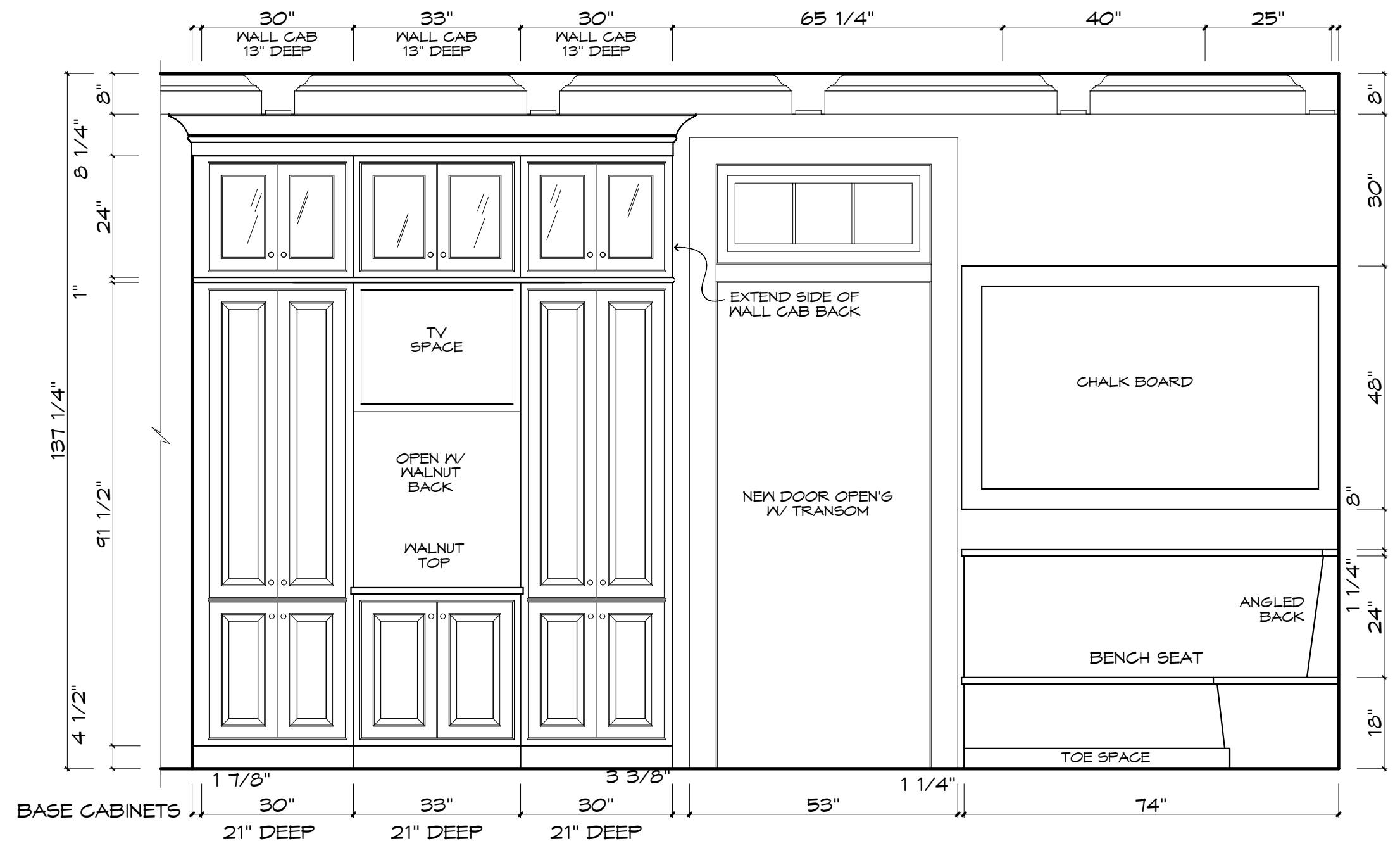
C PANTRY WALL ELEVATION SCALE: 1/2" = 1'-0"
