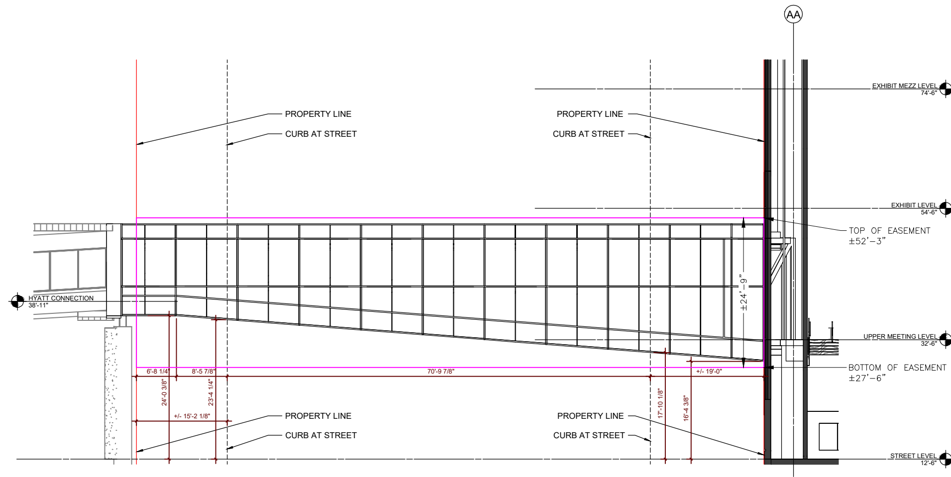
1 VEL R. PHILLIPS AVE SKYBRIDGE AIR RIGHTS EASEMENT SECTION NOT TO SCALE
