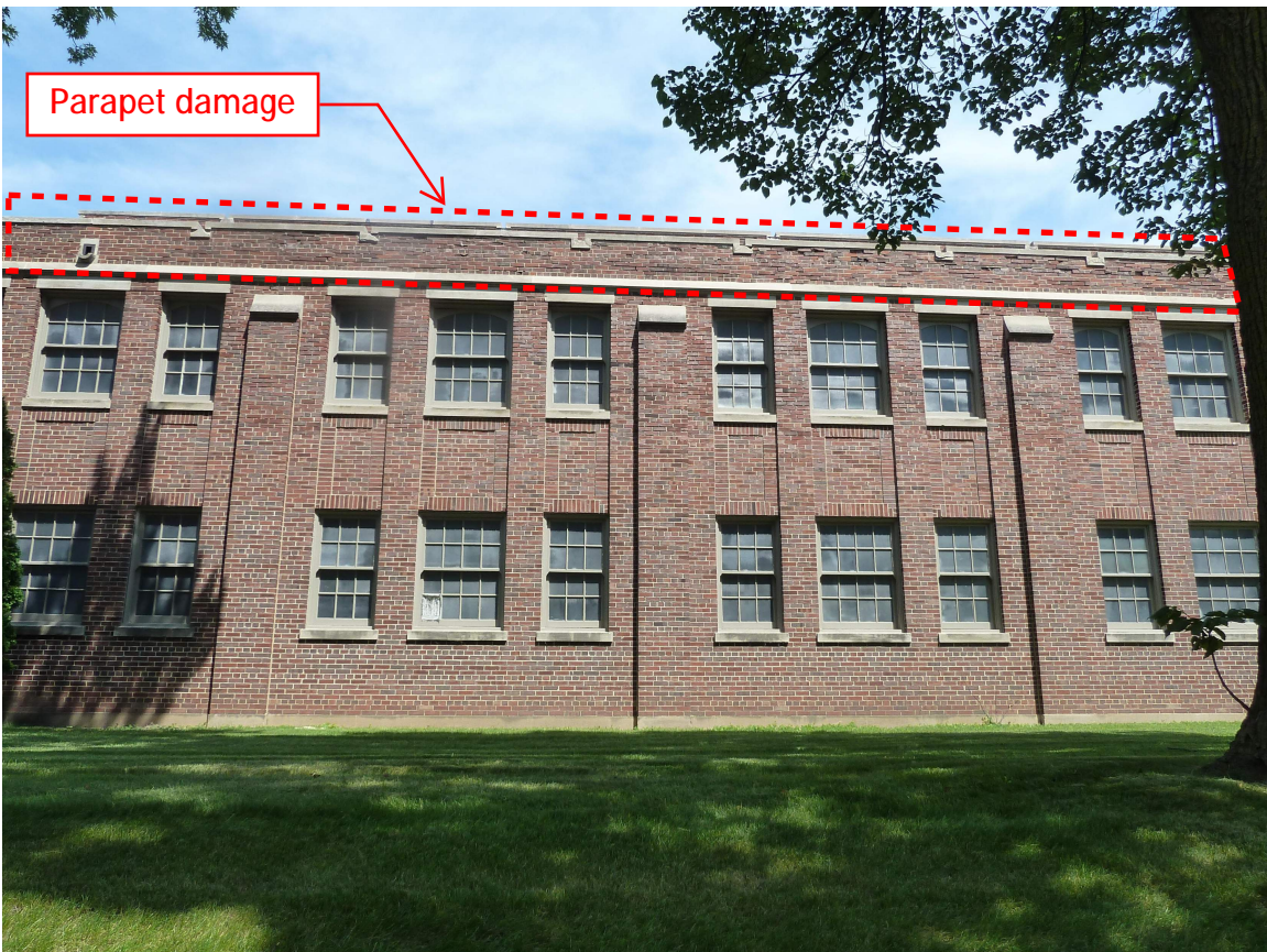
Photo 13 - West (central portion) at Gymnasium
