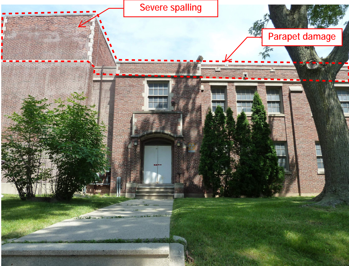
Photo 14 - West (northern portion) at Gymnasium
