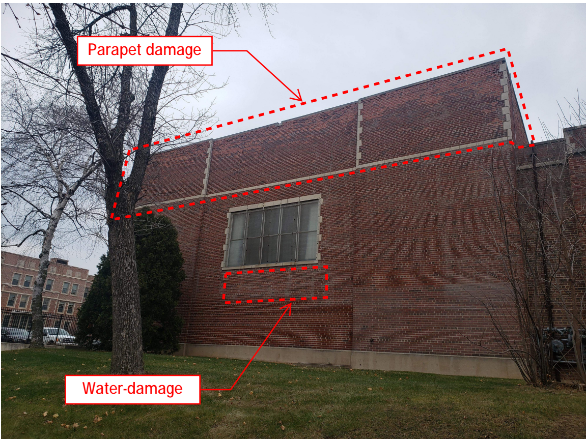
Photo 24 - West Overall at Pool Addition
