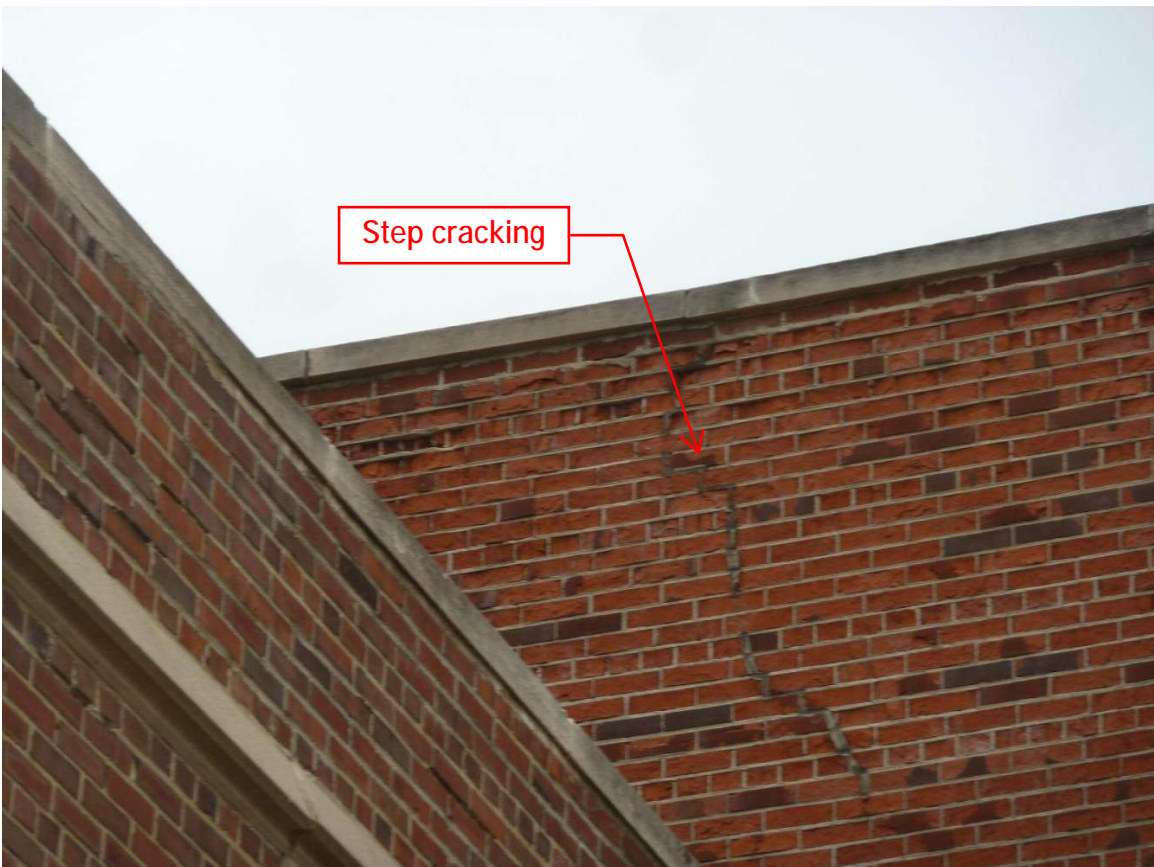
Photo 34 - South-east elevation cracking at Pool Addition
