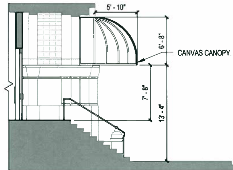
2 SECTION-BROADWAY ENTRANCE 1/8" = 1'-0"
