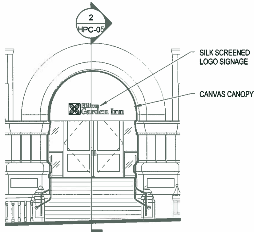
1 PARTIAL EAST ELEVATION 1/8" = 1'-0"
