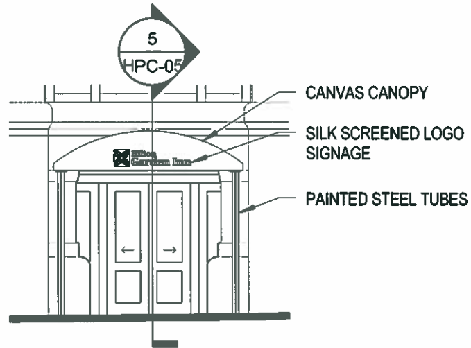
4 PARTIAL SOUTH ELEVATION 1/8" = 1'-0"
