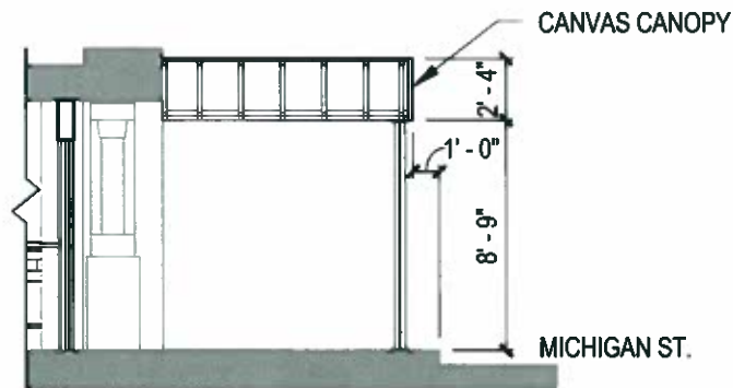
5 SECTION-MICHIGAN ST ENTRANCE 1/8" = 1'-0"
