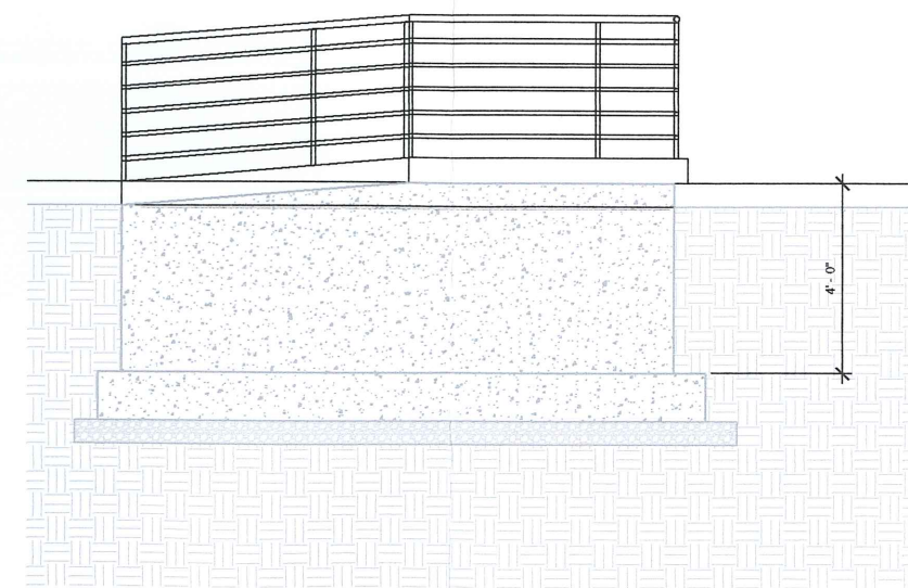
4 Foundation section 1/2" = 1'-0"
