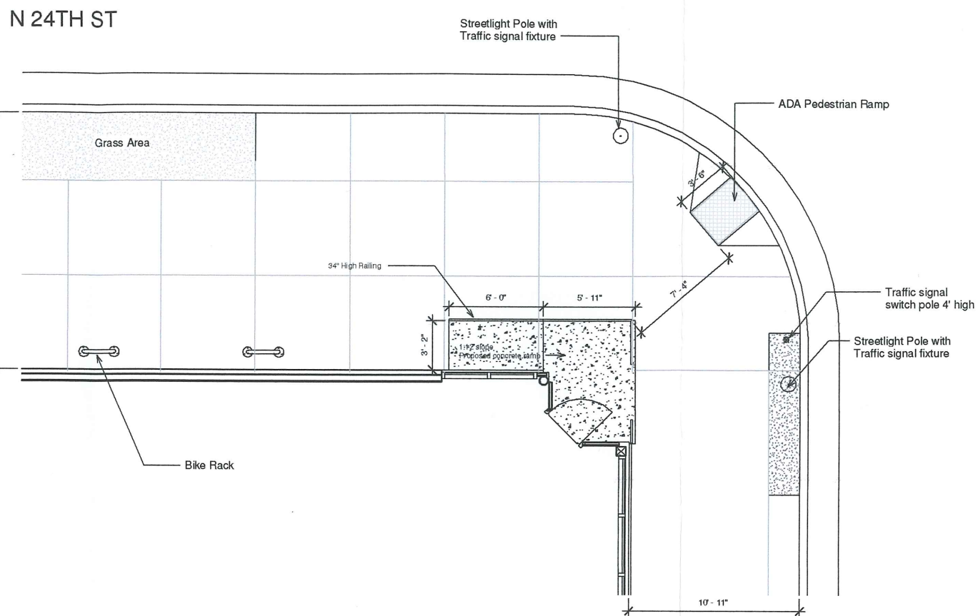
3 Level 1 - PROPOSED RAMP 1/4" = 1'-0"
