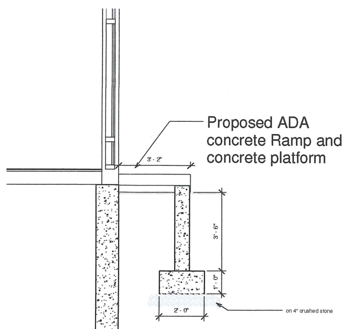
3 Level 1 - PROPOSED RAMP 1/4" = 1'-0"
