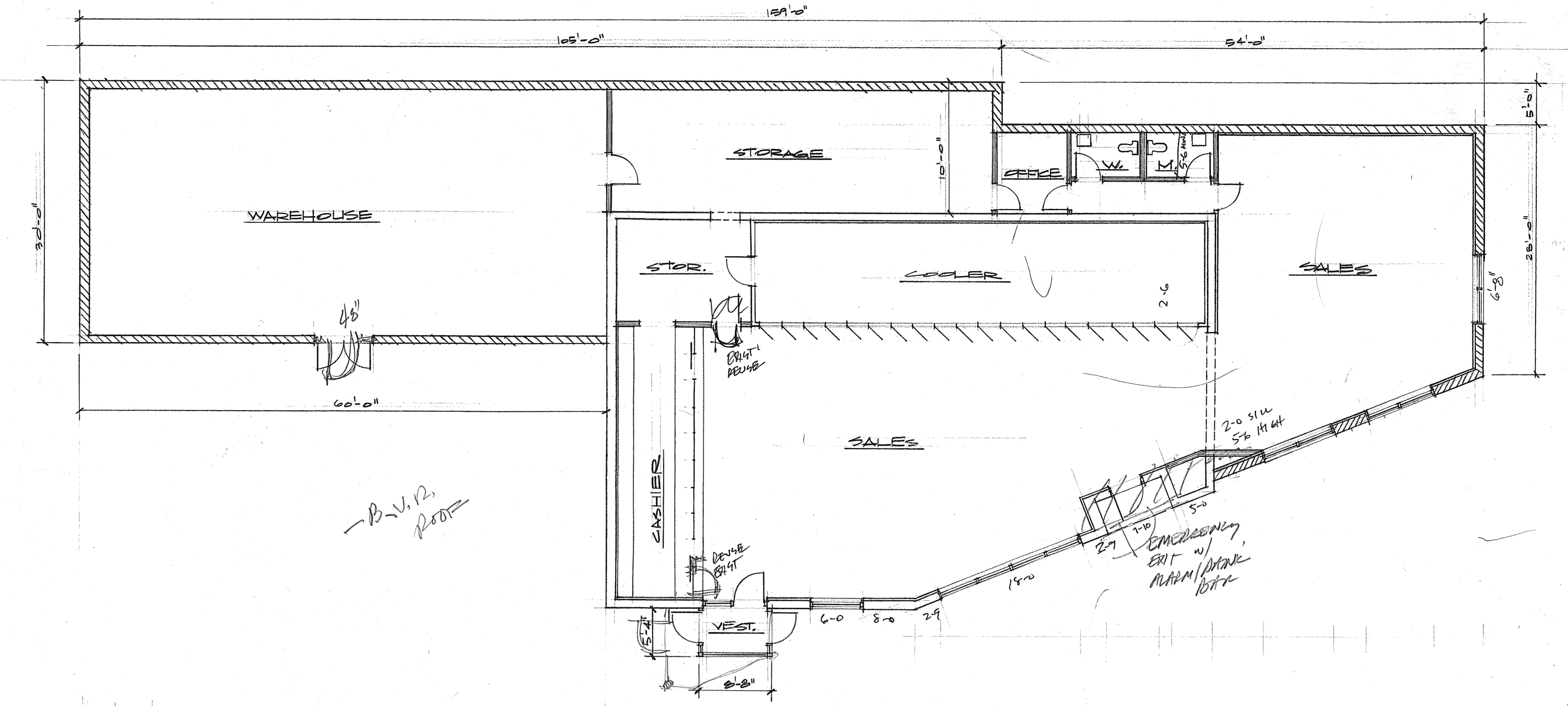
Floor Plan 1/8" = 1'-0"
