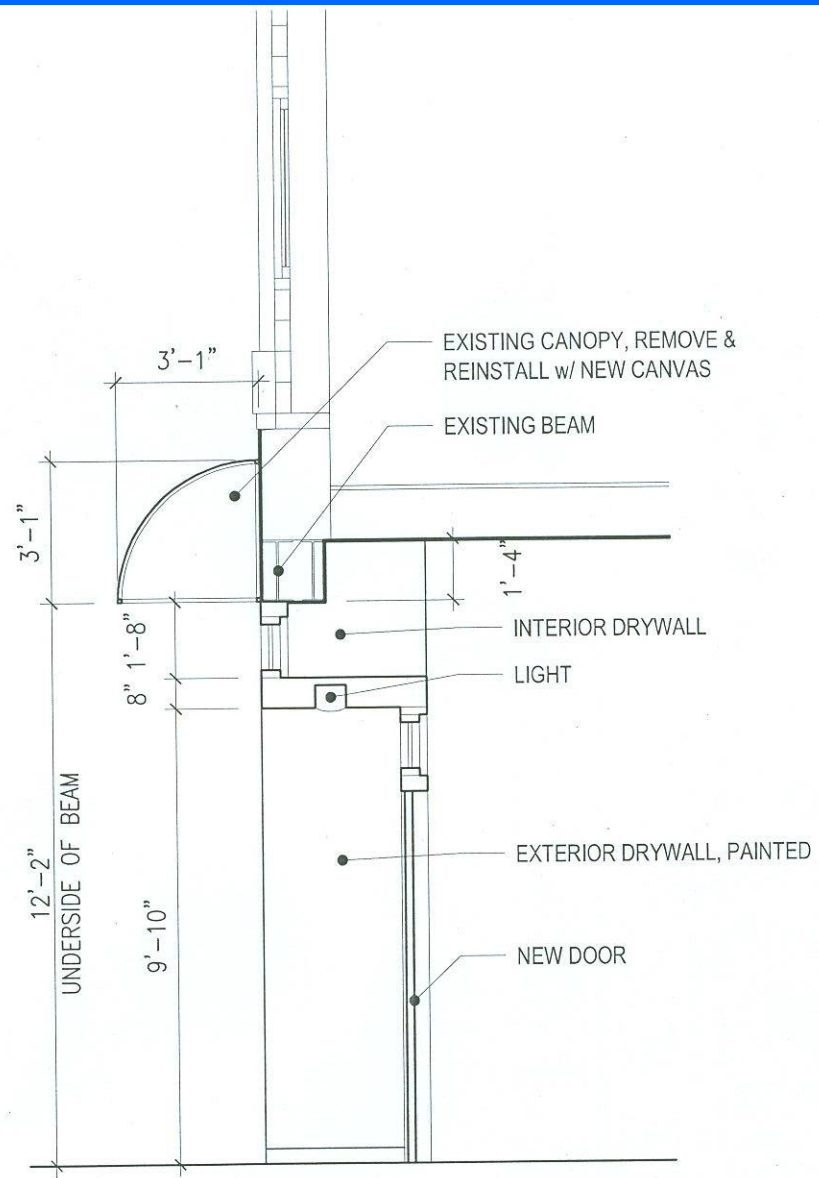
2. SECTION
