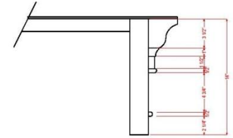
Detail 3 / 3
