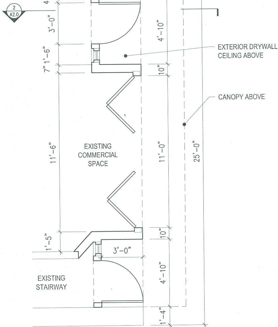
1. PLAN
