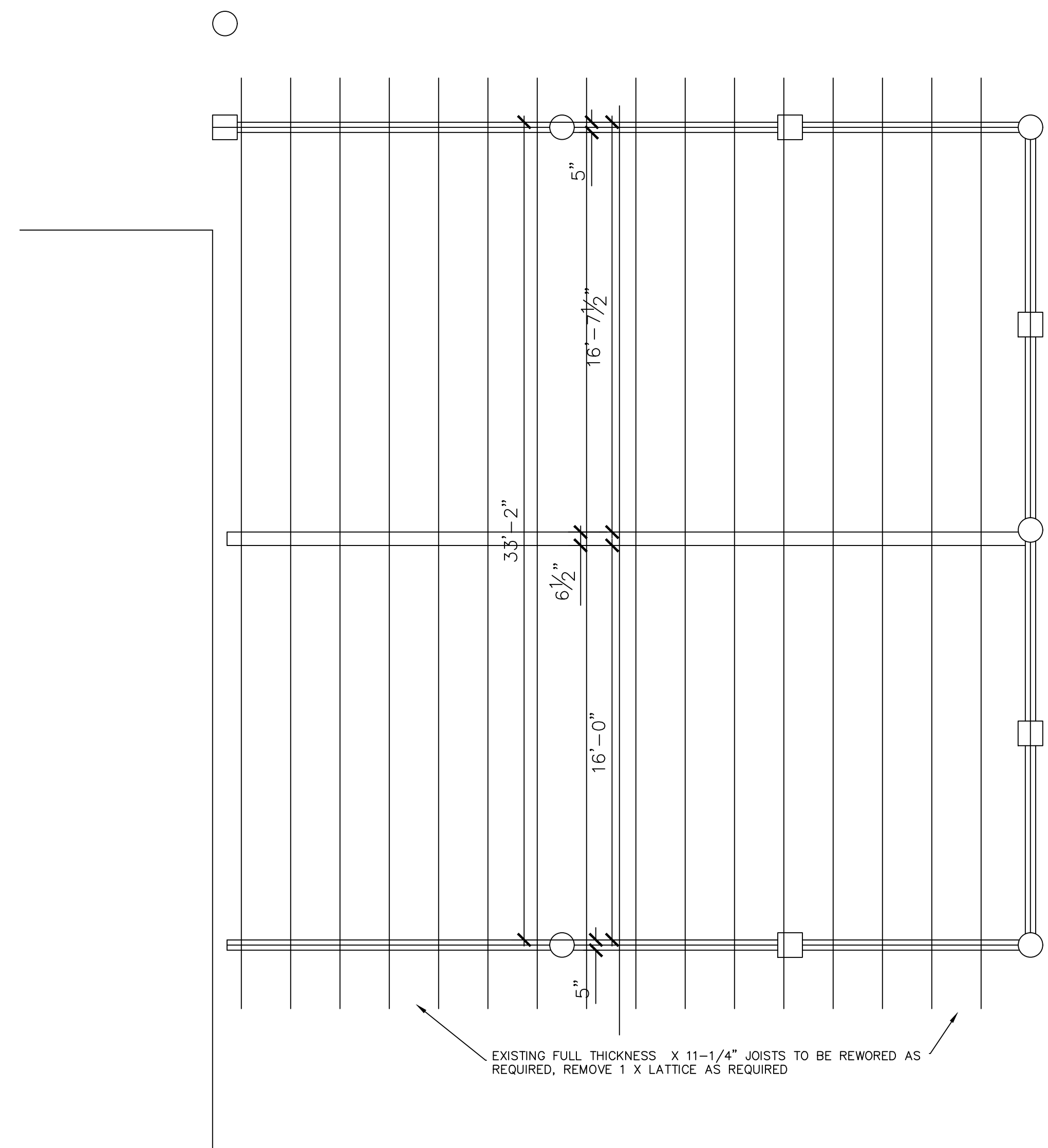
EXISTING LAYOUT
