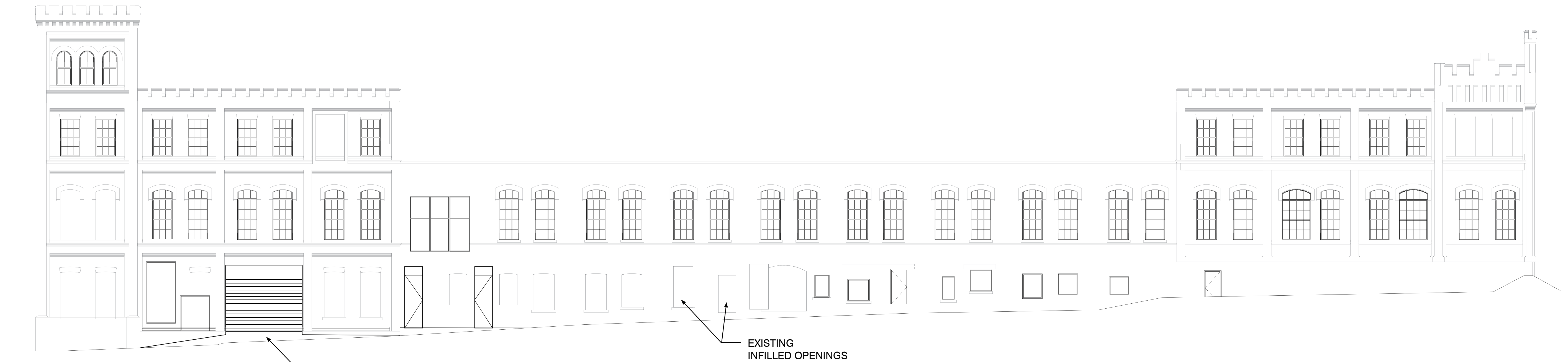
NORTH ELEVATION
