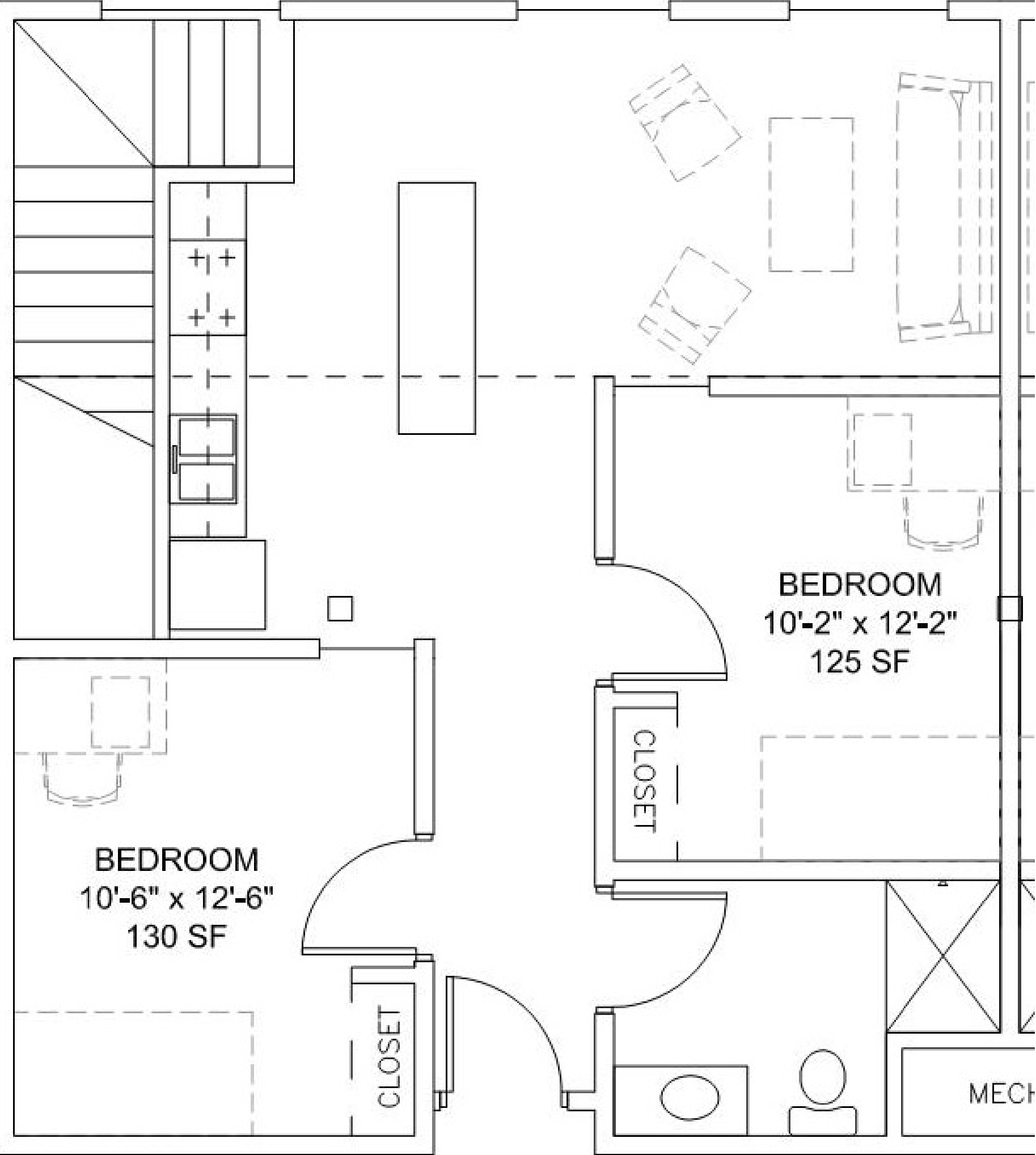
UNIT Q2 PLAN (LOWER) TYP
