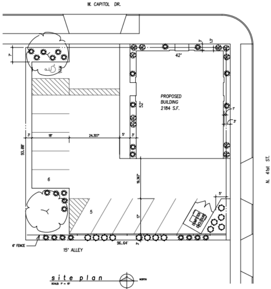
Restaurant Elevation and Site Plan
