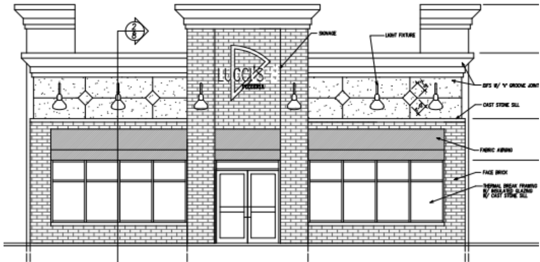
Capitol Drive Elevation
