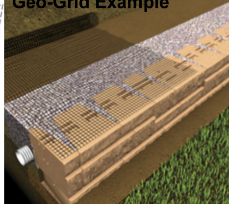
Geo-Grid Example
