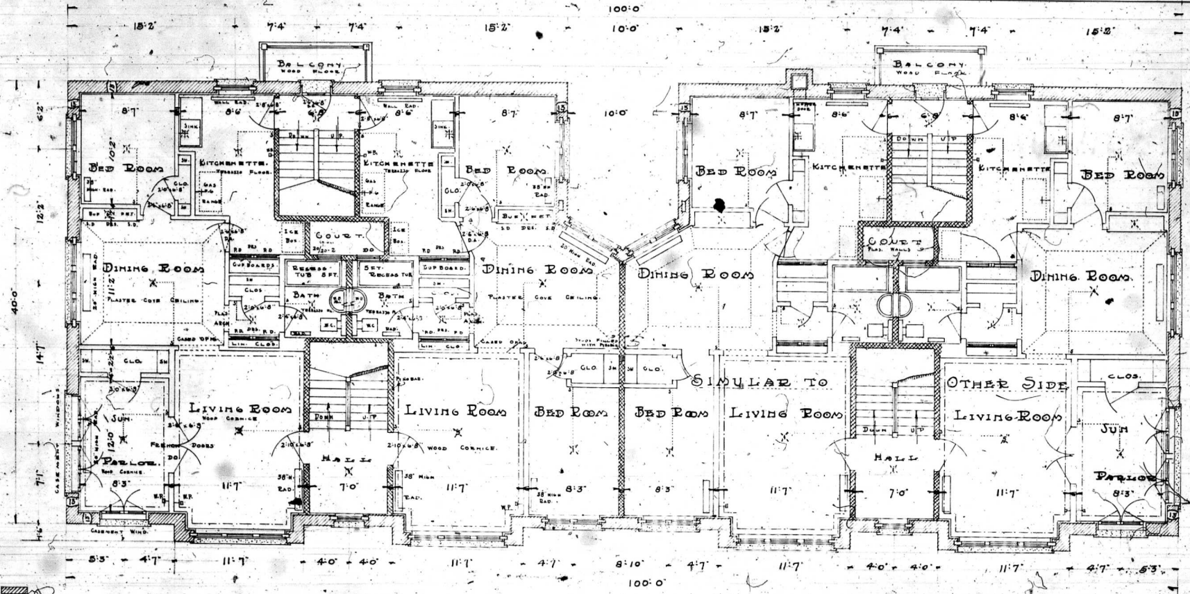
SECOND & FIRST FLOORS Wm. Hoffman Builder
