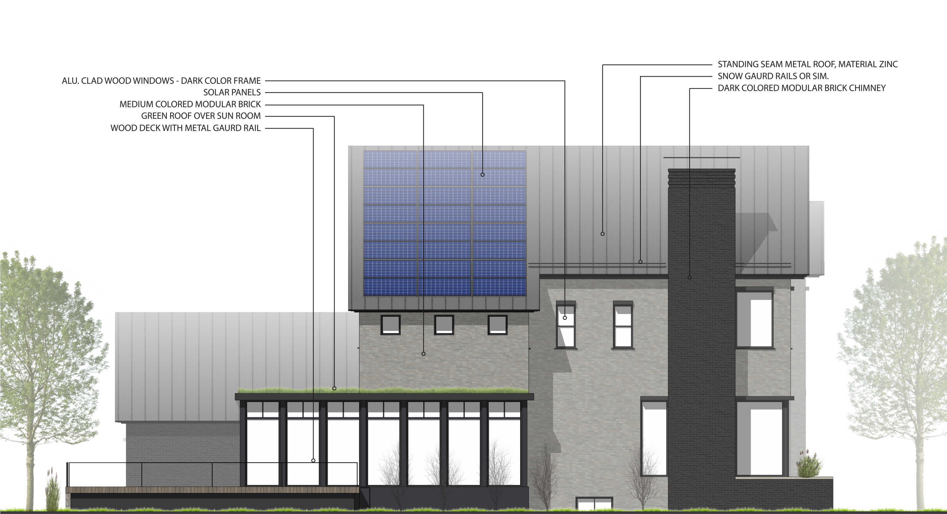
SOUTH ELEVATION
