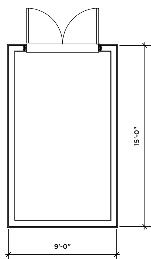
PLAN
