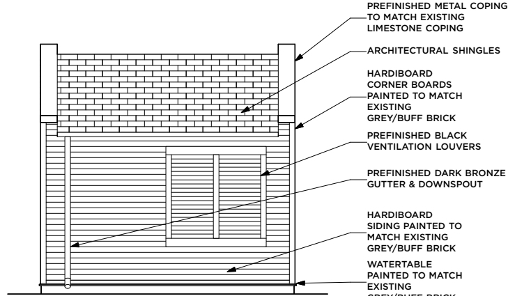
WEST ELEVATION
