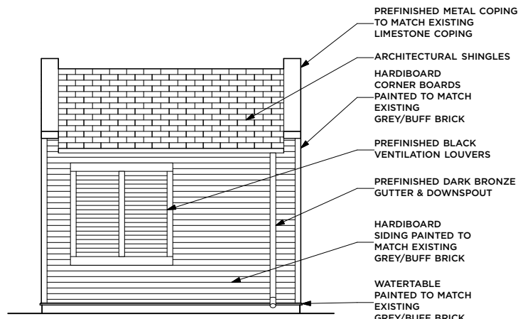
EAST ELEVATION
