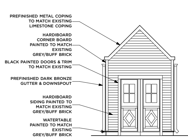
NORTH ELEVATION
