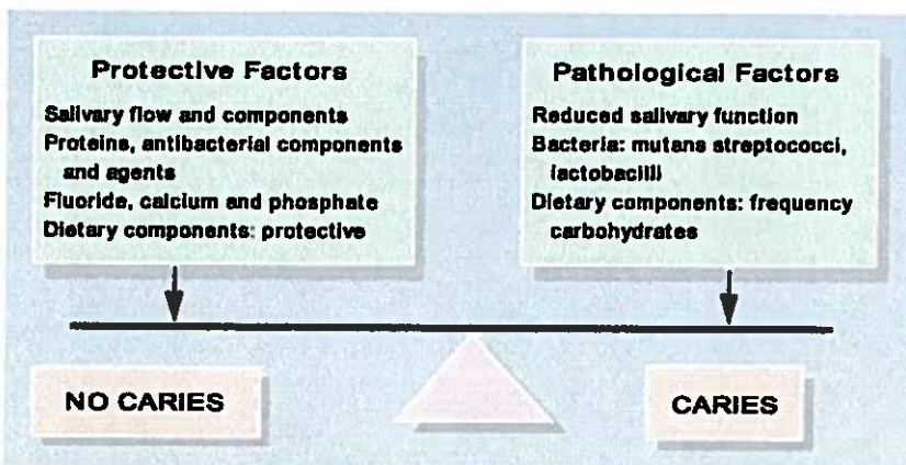
Figure 5. The caries balance: a schematic diagram of the balance between pathological and protective factors in the caries process. (Reproduced from Featherstone 1 with permission of the publisher. Copyright ©1999, Munksgaard.)
