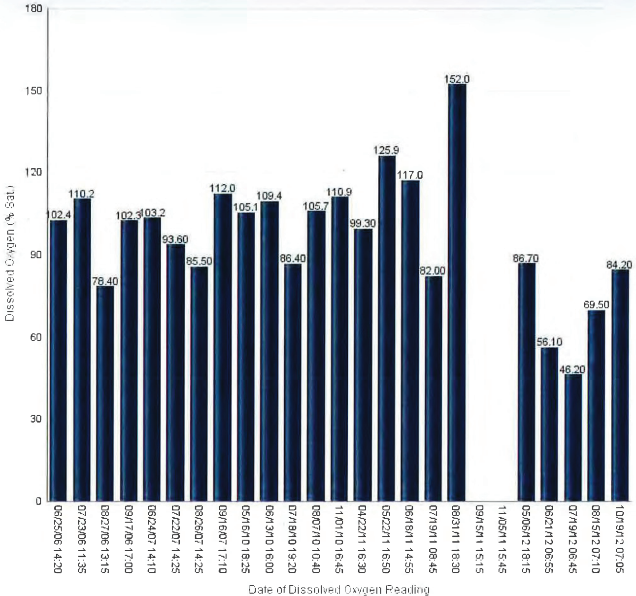
Measured Dissolved Oxygen (% Sat.)
