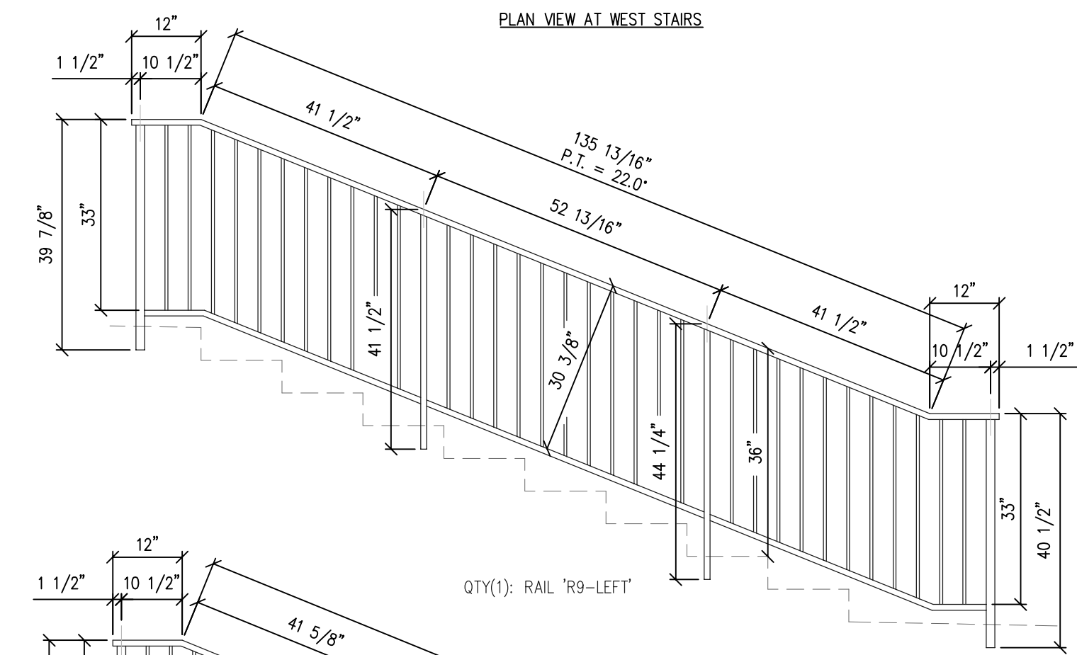
PLAN VIEW AT WEST STAIRS
