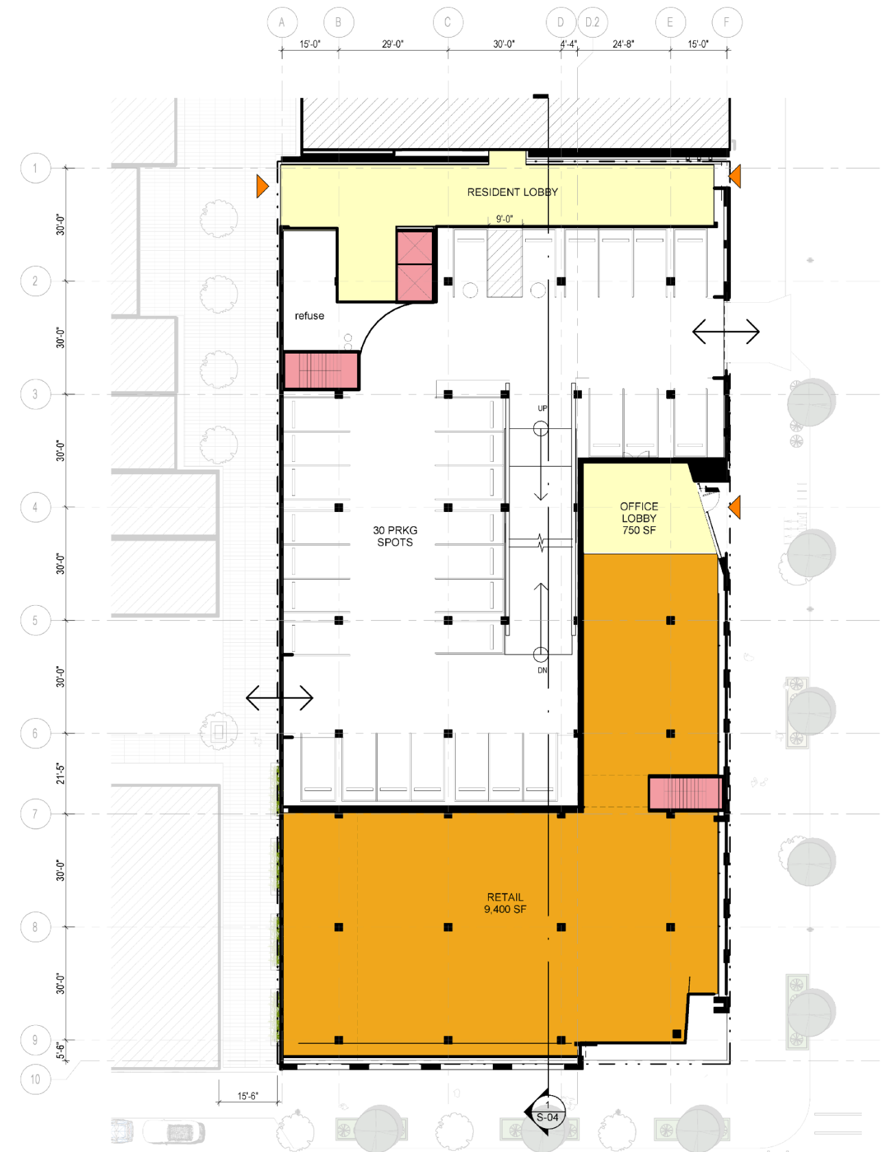
LEVEL ONE / GRADE
