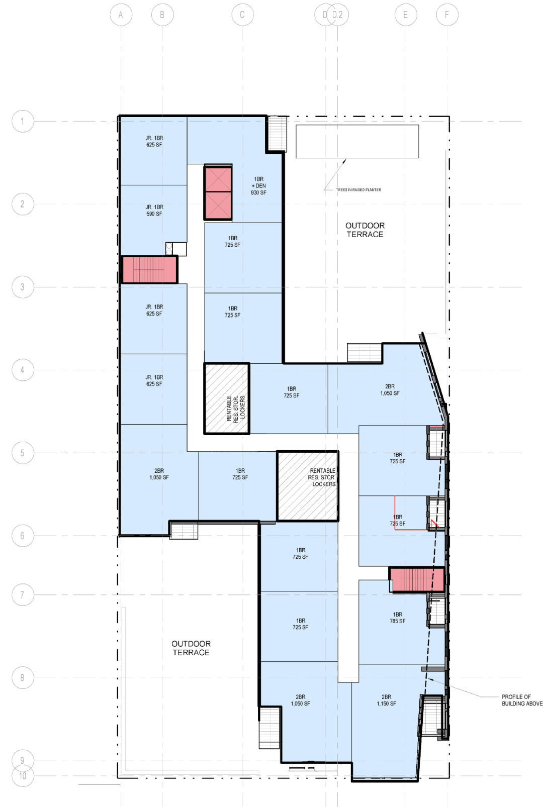
TYP. LEVEL FLOORS 5-7 (FLOOR 8 NOT SHOWN)
