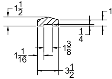
HANDRAIL
