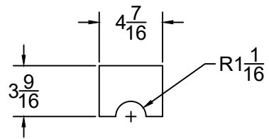
RAILING SPACER 1-1/8 THICK
