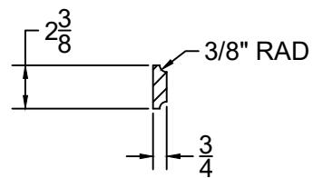
RAILING TOE RAIL
