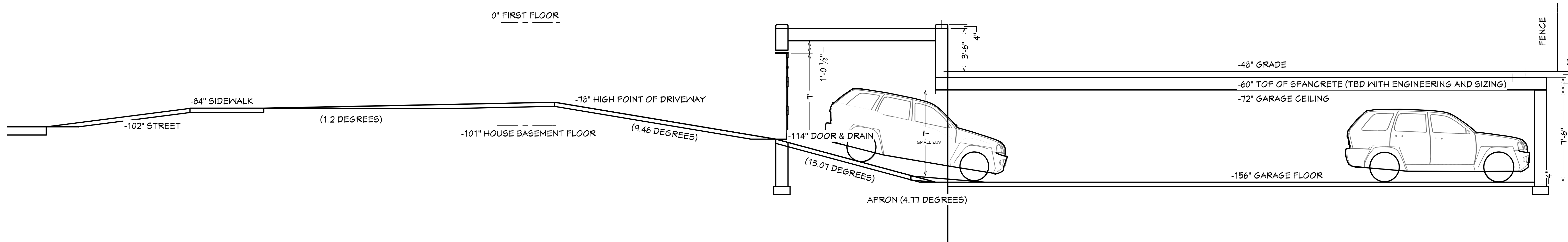
S1 CROSS SECTION AT DRIVEWAY AND GARAGE ENTRY 1/4 IN = 1 FT
