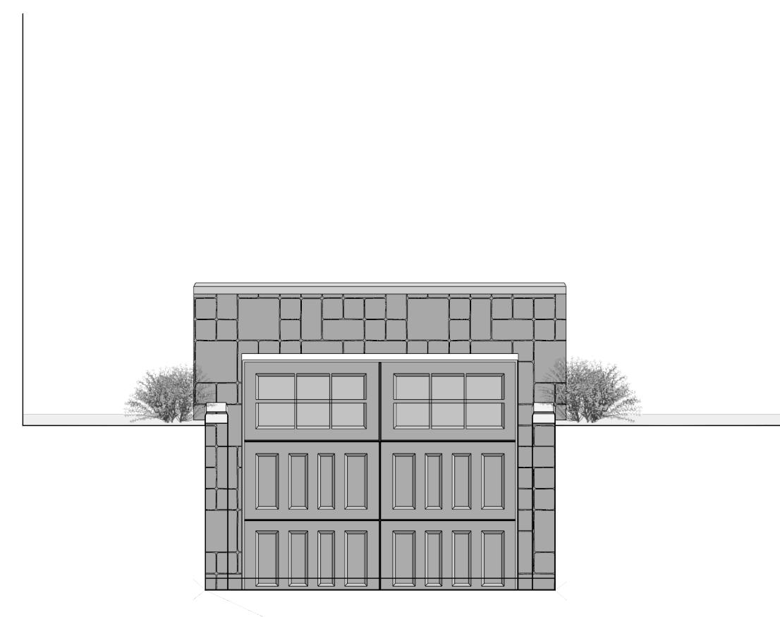
S2 WEST ELEVATION 1/4 IN = 1 FT
