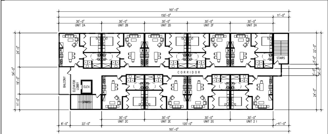
Floorplans, Floor 2 to 4,
