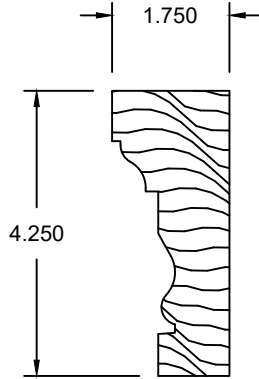
3 1/2" Brickmold with Backband
