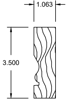
3-1/2" Brickmold (all products)
