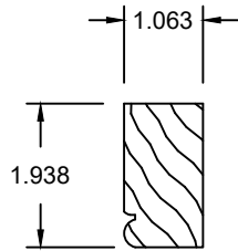
2" Beaded Casing
