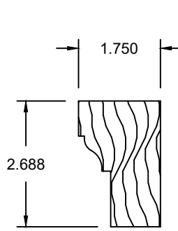
1-15/16" Flat Casing with Backband
