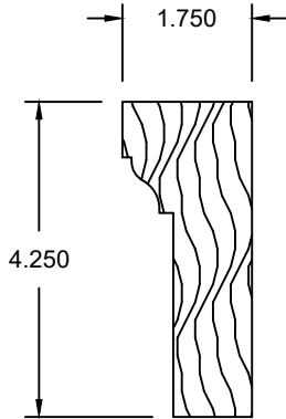
3 1/2" Flat Casing with Backband (all products)
