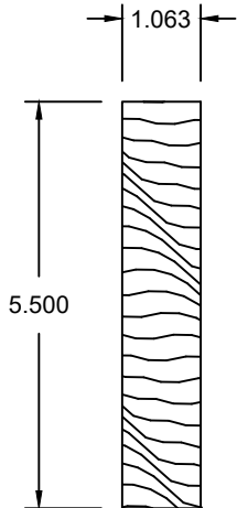
5-1/2" Flat Casing
