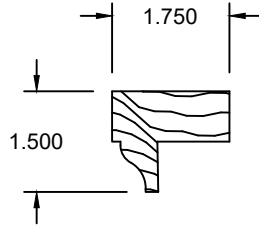
Backband Casing (all products)
