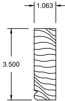
3-1/2" Beaded Casing
