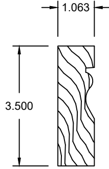
3-1/2" Flat Casing (all products)
