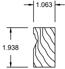
1-15/16" Brickmold (all products)
