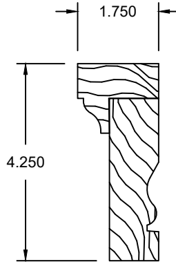
3-1/2" Flat Casing with Backband - 2 piece (all products)
