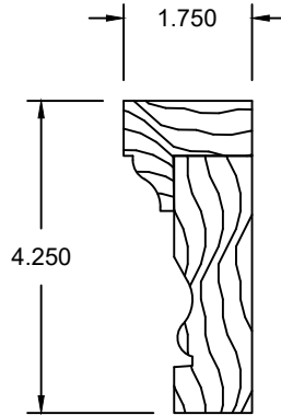
3-1/2" Brickmold with Backband - 2 piece (all products)
