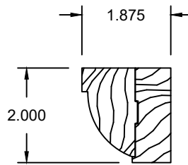
Prospect Casing
