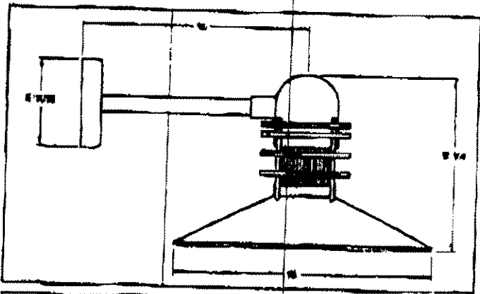
WPLS-41PR-16 16" Side Mount Reflector. Shown With WM-GN10-SPI Pipe Bracket.
