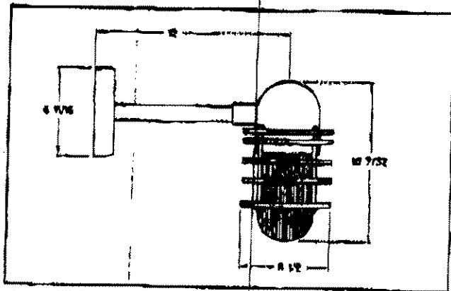
WPLSNR Side Mount Fixture with No Reflector. Shown With WM-GNB-SPI Pipe Bracket.
