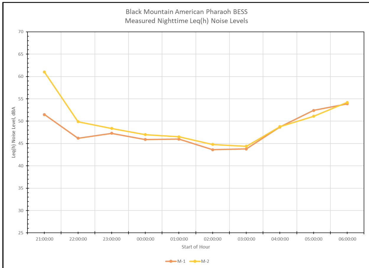
Figure 3. Measured L_{eq}(h) Ambient Noise Levels
