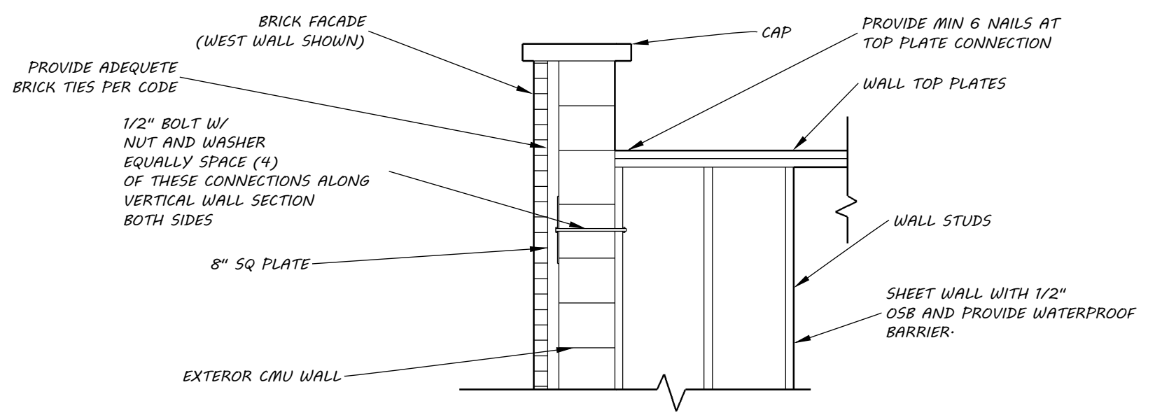
2 WALL CONNECTION A4 1/2" = 1'-0"
