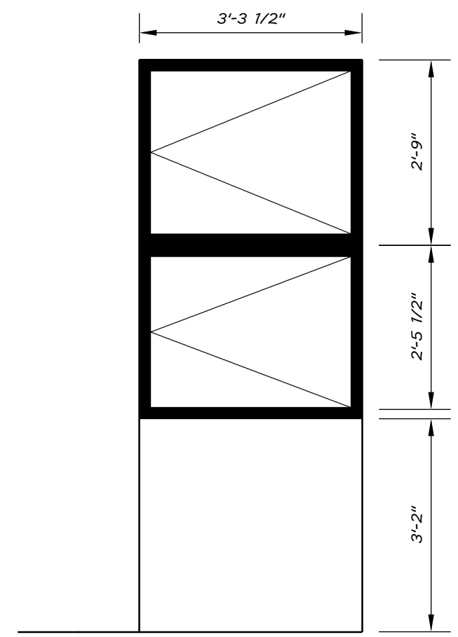
3 ENTRY GLASS ELEVATION A4 1/4" = 1'-0"
