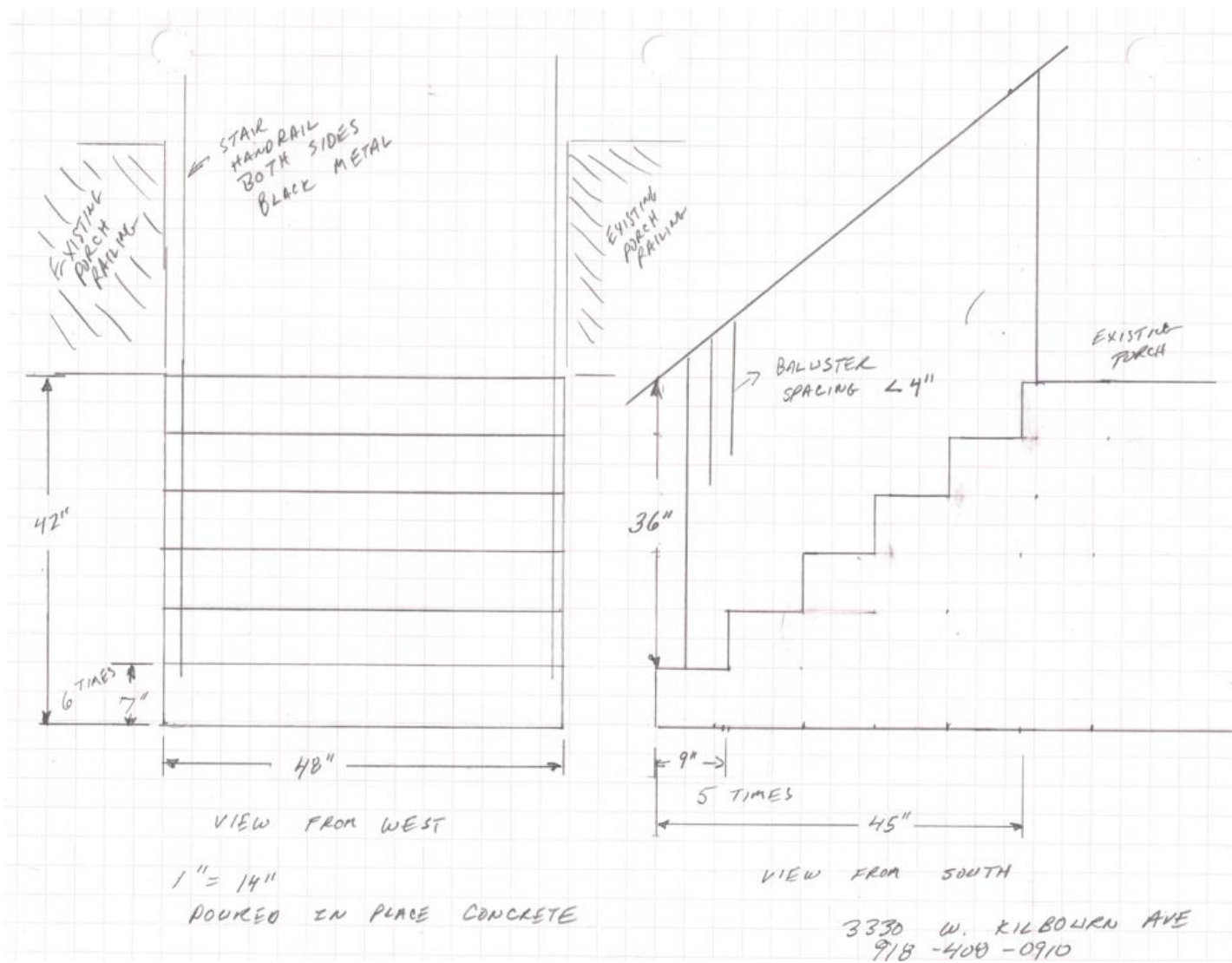
Step and railing plans
