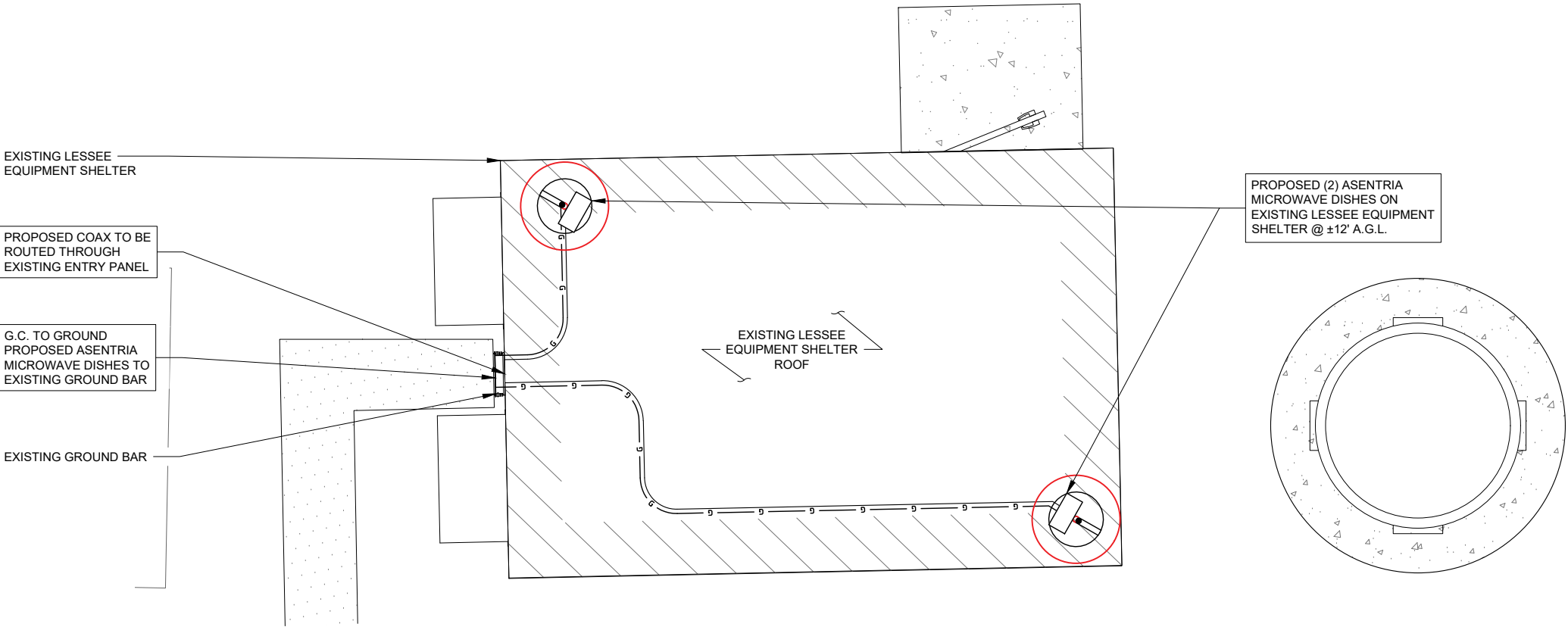
1 SHELTER PLAN SCALE: 1" = 2'
